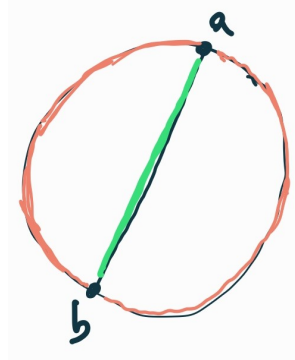
Figure 4.16: TODO: make the final picture not go through the center, change the label for the points to e_1 and e_2
