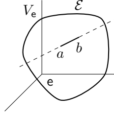
Figure 4.6: \mathcal{E} is the ensemble space and V_e is the embedding vector space with origin e . Any affine line, like the dashed one in the picture, will intersect \mathcal{E} over a finite range limited by the two elements a and b of the vector space (but not necessarily of the ensemble space).
