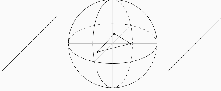
Figure 4.5: Affine vs convex set. The ball is the ensemble space. The triangle represents a convex subset. The disc containing the triangle is the affine closure of the triangle in the ensemble space. The plane is the affine closure/span of the triangle in the embedding vector space centered at one of the three ensembles.
