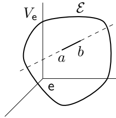
Figure 4.7: \mathcal{E} is the ensemble space and V_e is the embedding vector space with origin e . Any affine line, like the dashed one in the picture, will intersect \mathcal{E} over a finite range limited by the two elements a and b of the vector space (but not necessarily of the ensemble space).
