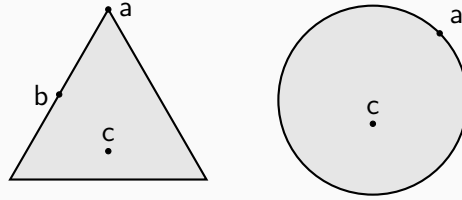
Figure 4.3: In both spaces, \mathbf{a} is an extreme point while \mathbf{c} is an internal point; \mathbf{b} is a boundary point, but is not an extreme point (it is the mixture of the vertices on the same side). On the circle, all boundary points are extreme points.
