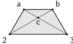
Figure 4.13: Cut triangle.
