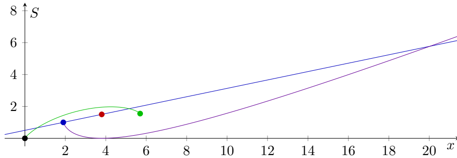
Figure 4.7: Visual representation of the bounds. See proof for details.
