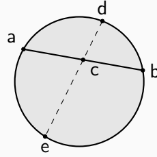
Figure 4.17: The set \{a, b\} is componential, but its convex hull (the segment) is not: c is in the convex hull but can be decomposed into d and e , which lie outside of the hull.
