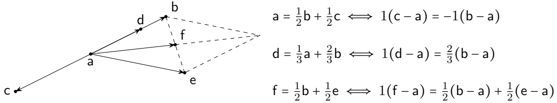
Figure 4.4: Once a reference point is picked (i.e. a in the figure), the differences with respect to that point behave like elements of a vector space. The relationship between ensembles in terms of mixtures become vector space relationships between differences. Note that the sum is effectively a “half parallelogram law,” so that the result always is a member of the convex space.
