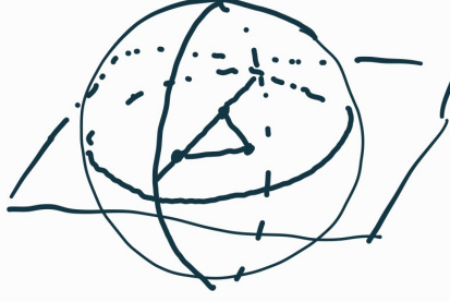
Figure 4.5: Affine vs convex set. The ball is the ensemble space. The triangle represents a convex subset. The disc containing the triangle is the affine closure of the triangle in the ensemble space. The plane is the affine closure/span of the triangle in the embedding vector space centered at one of the three ensembles.
