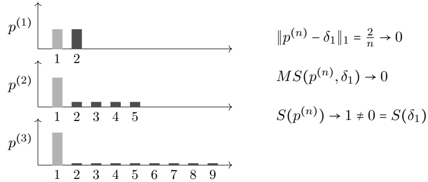
Figure 4.15: A vanishing fraction of probability mass spread over exponentially many outcomes. The distributions converge to \delta_1 in \ell^1 /total variation/Jensen–Shannon divergence, but the entropy does not converge.
