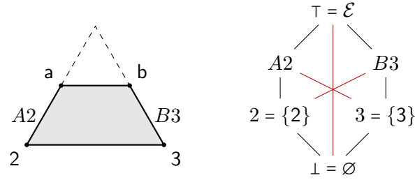
Figure 4.12: On the left, the cut triangle. On the right, the lattice of the orthogonal subspaces. The red lines connect the orthogonal complements.
