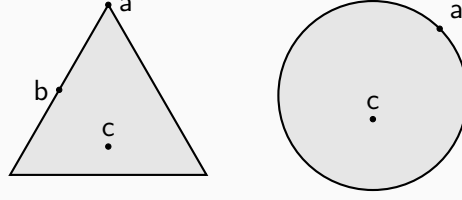
Figure 4.2: In both spaces, a is an extreme point while c is an internal point; b is a boundary point, but is not an extreme point (it is the mixture of the vertices on the same side). On the circle, all boundary points are extreme points.
