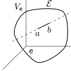
Figure 4.6: \mathcal{E} is the ensemble space and V_e is the embedding vector space with origin e . Any affine line, like the dashed one in the picture, will intersect \mathcal{E} over a finite range limited by the two elements a and b of the vector space (but not necessarily of the ensemble space).
