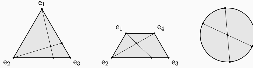
Figure 4.3: Examples for mono- and multidecomposability.
