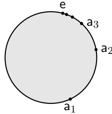
Figure 4.9: Discontinuity of fraction.
