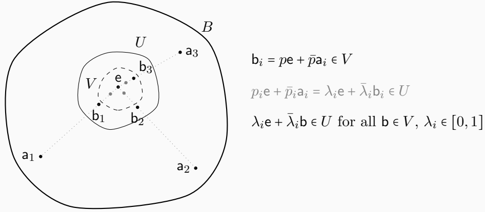
Figure 4.1: Boundedness shrinks all of A into the neighborhood V (giving the b_i ); the tube lemma guarantees that any further mixture of e with a point of V stays in U (giving the gray points).
