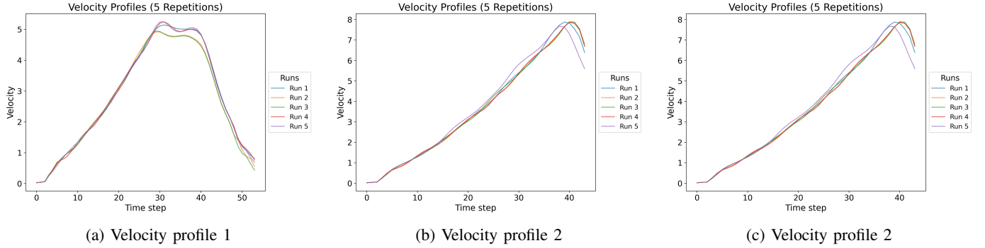
Fig. 4: (Autoware) Overview of velocity profiles from reexecution of random scenario 5 times. The profiles reveal no significant deviation as indicated by the low fitness score variation in Figure 3.
