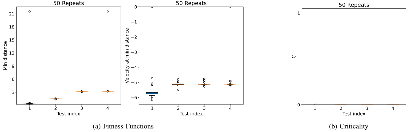
Fig. 3: (Autoware) Fitness variation by reexecuting randomly generated scenarios 50 times in the Carla-based HiFi simulator. Both distance fitness and velocity fitness variation are low and no variation of the tests outcome (Figure b)) can be observed indicating low simulation flakiness.
