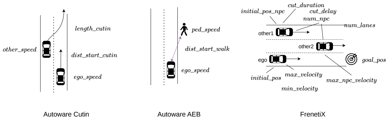
Fig. 2: Overview of scenarios and parameters used in the study: Cut-In scenario with and automated emergency breaking (AEB) scenario with a pedestrian in Autoware and a planning scenario in the FrenetiX case study. Names of parameters are for illustration purposes and can vary from the ones presented in the paper.
