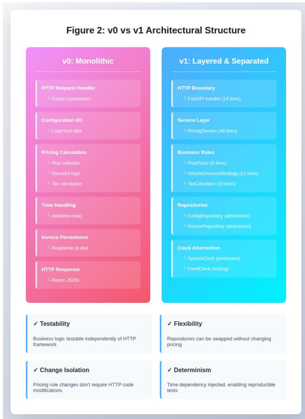
Figure 2: v0 vs v1 Architectural Structure – Layered design with explicit separation of concerns
