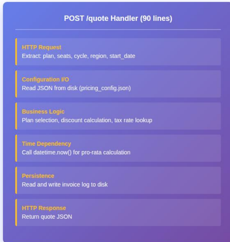
Figure 1: v0 Handler Coupling
