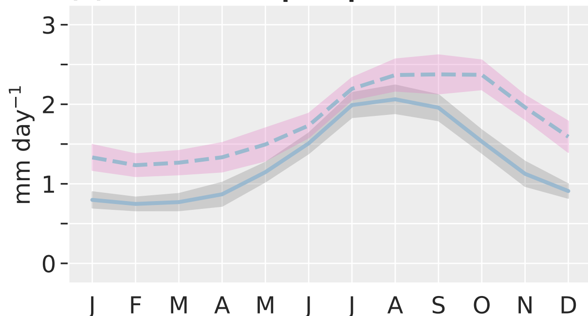
(f) Runoff
