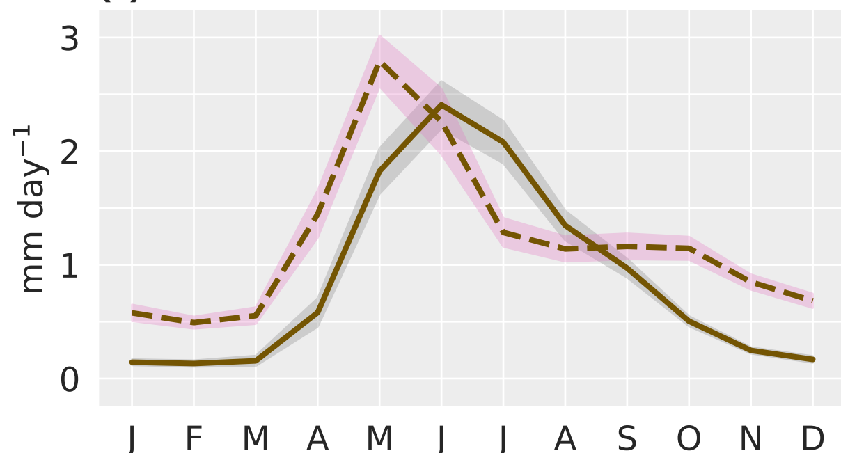
(g) Evapotranspiration
