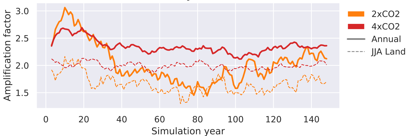
(b) Arctic amplification
