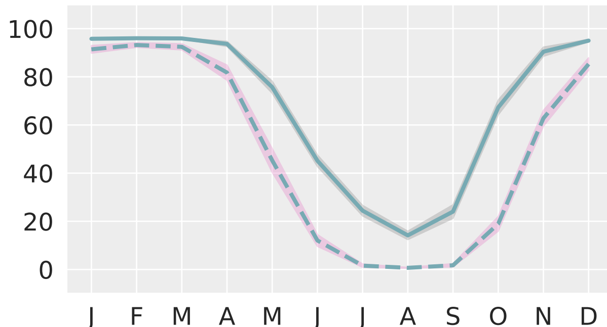
(c) Near-surface relative humidity
