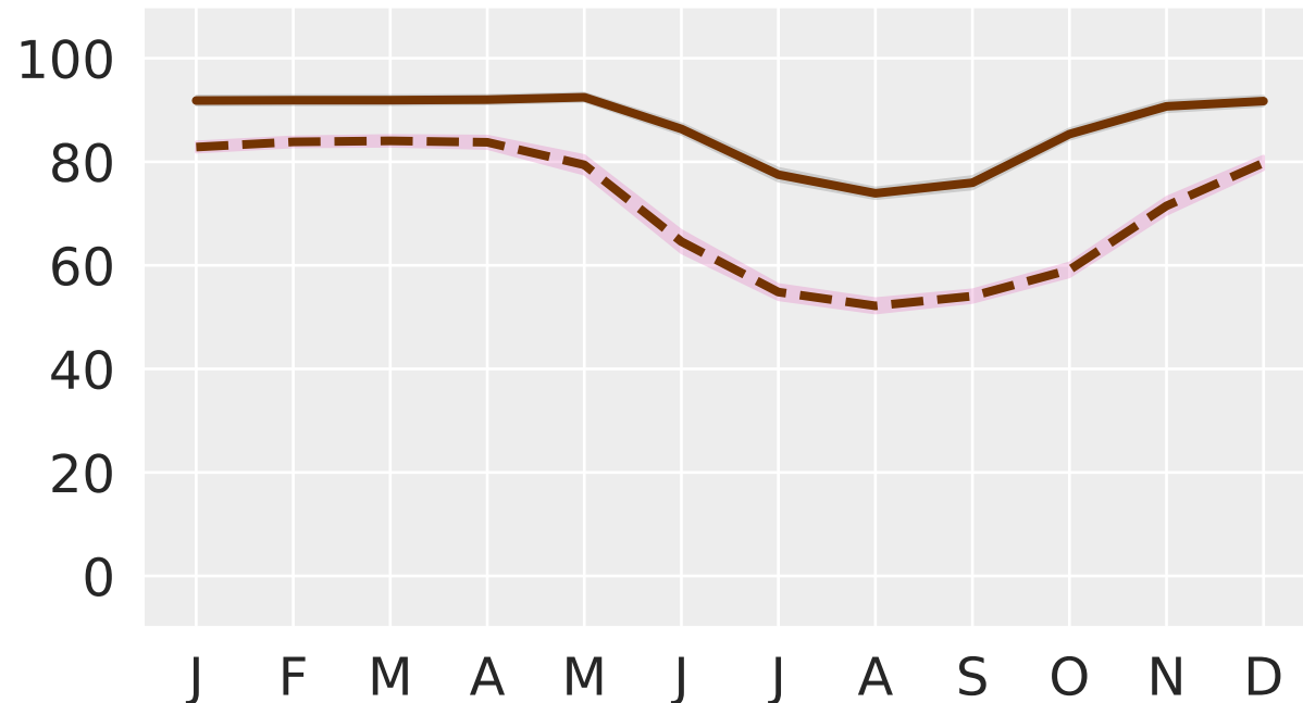
(b) Snow cover
