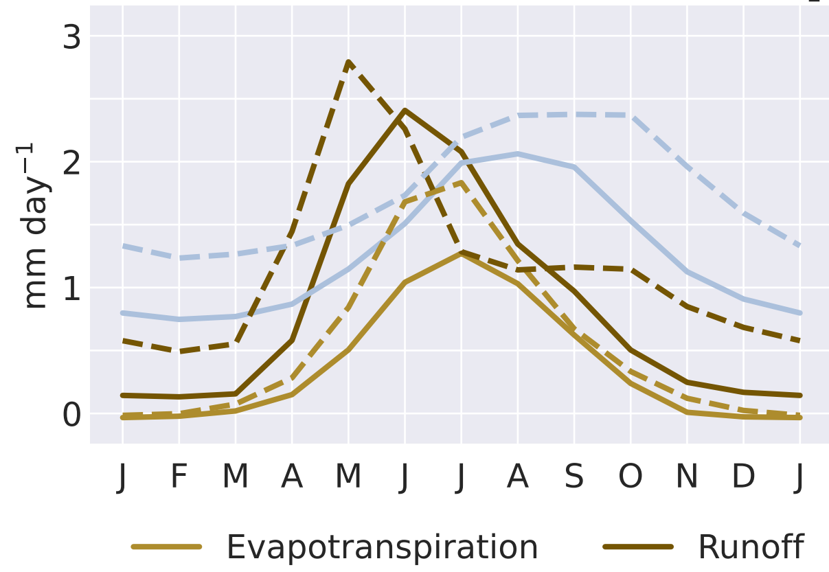
(b) Fluxes
