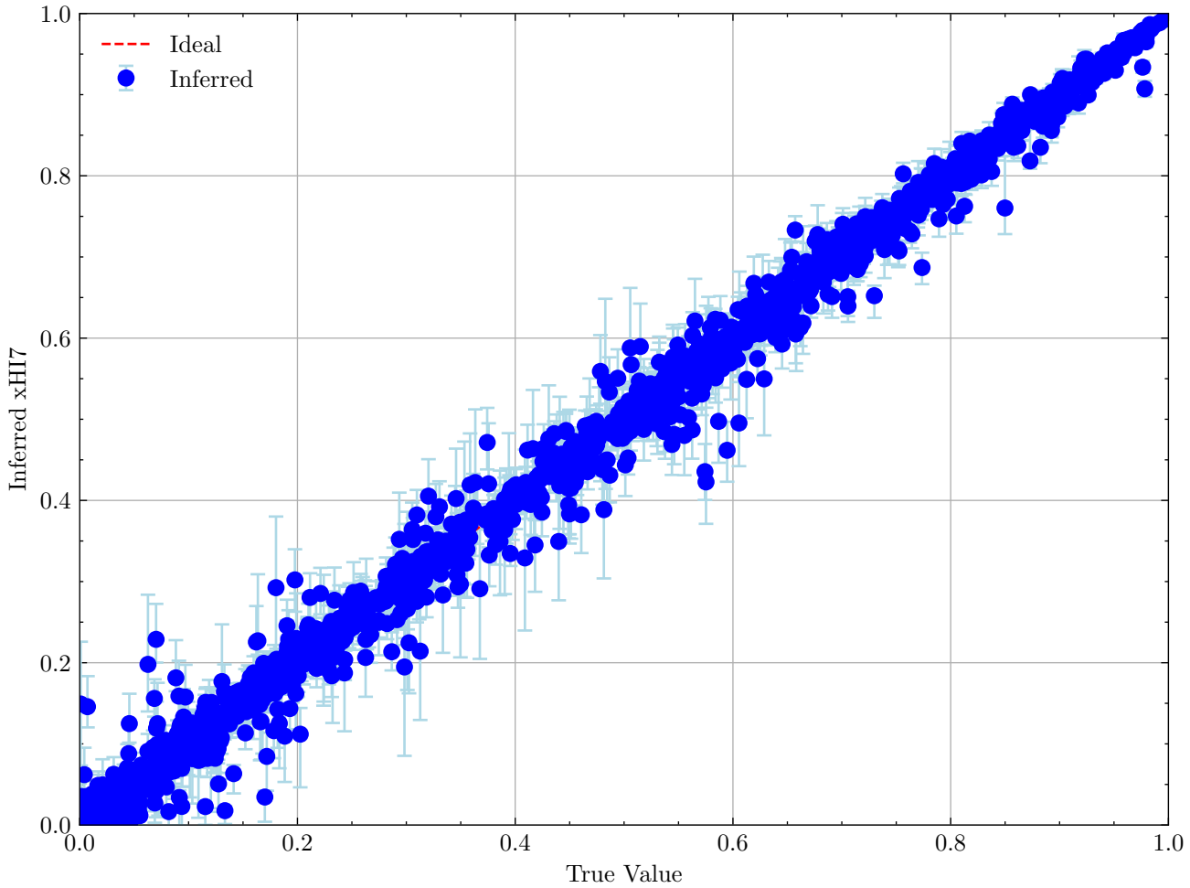
Calibration Scatter Plot for xHI7
