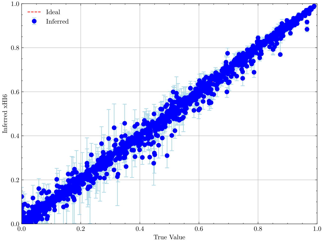
Calibration Scatter Plot for xHI6
