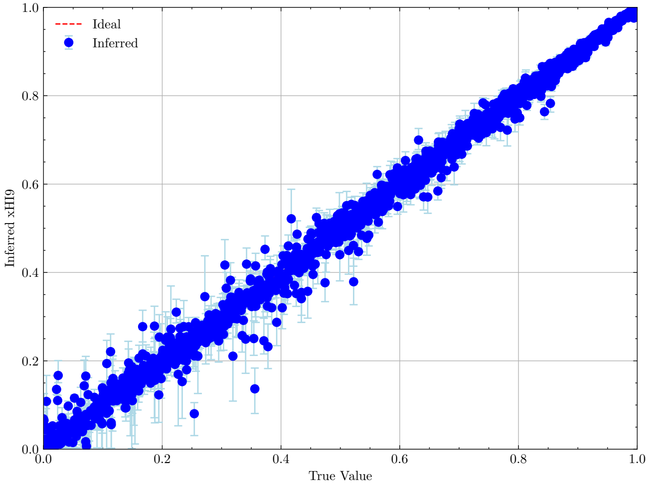
Calibration Scatter Plot for xHI9
