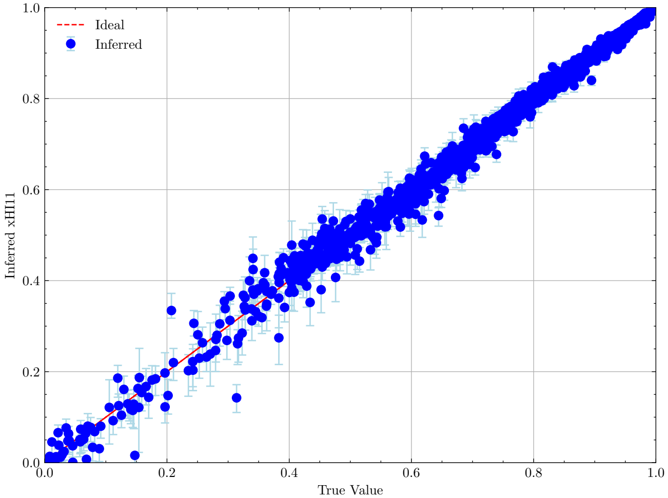
Calibration Scatter Plot for xHI11
