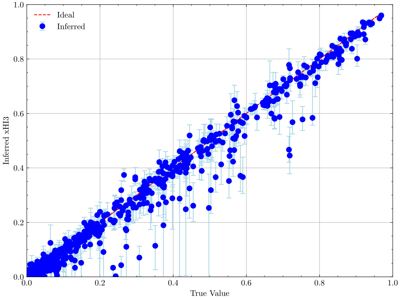
Calibration Scatter Plot for xHI3
