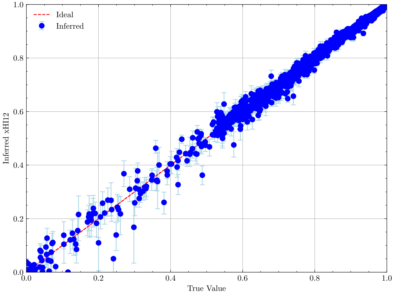
Calibration Scatter Plot for xHI12
