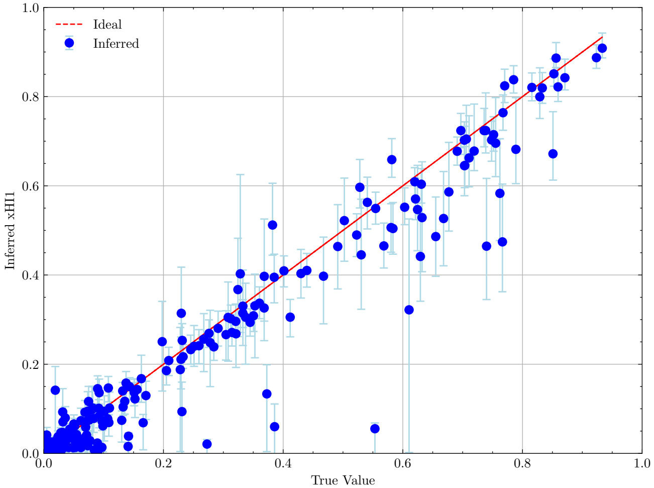
Calibration Scatter Plot for xHI1
