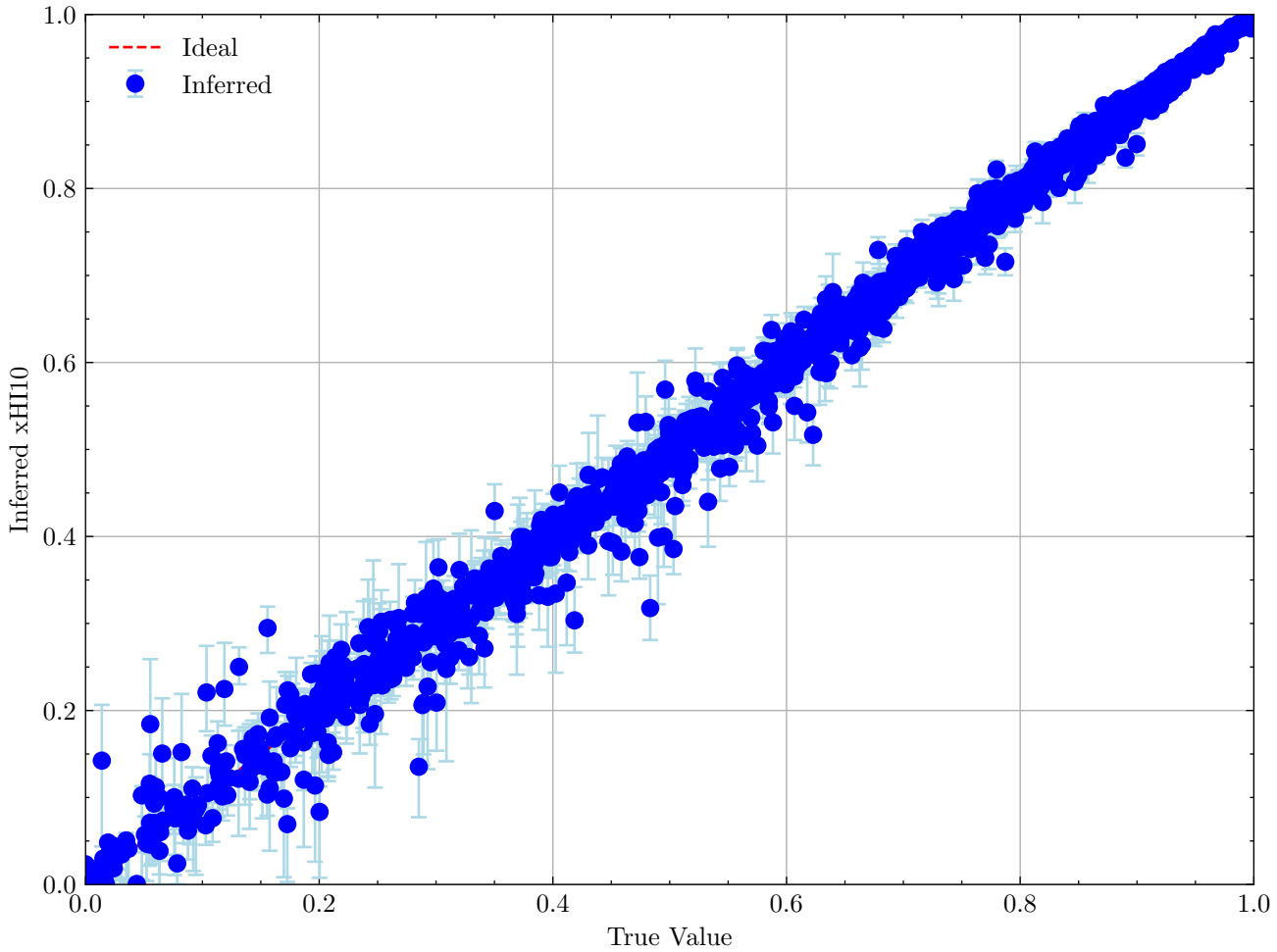
Calibration Scatter Plot for xHI10
