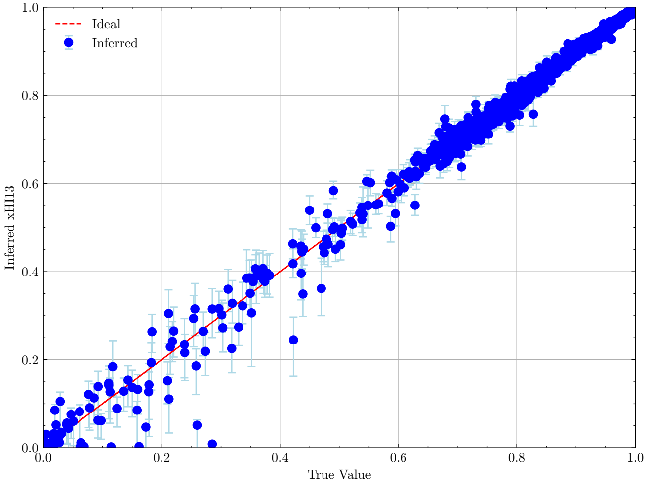
Calibration Scatter Plot for xHI13
