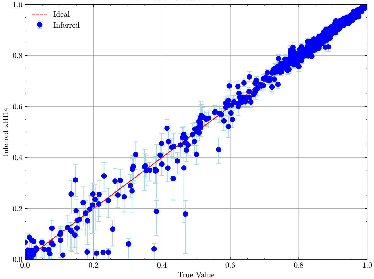
Calibration Scatter Plot for xHI14
