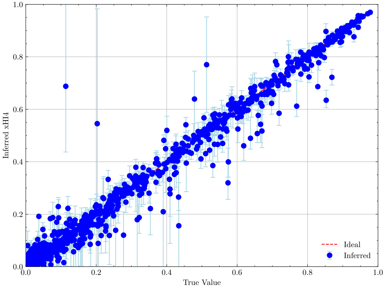
Calibration Scatter Plot for xHI4
