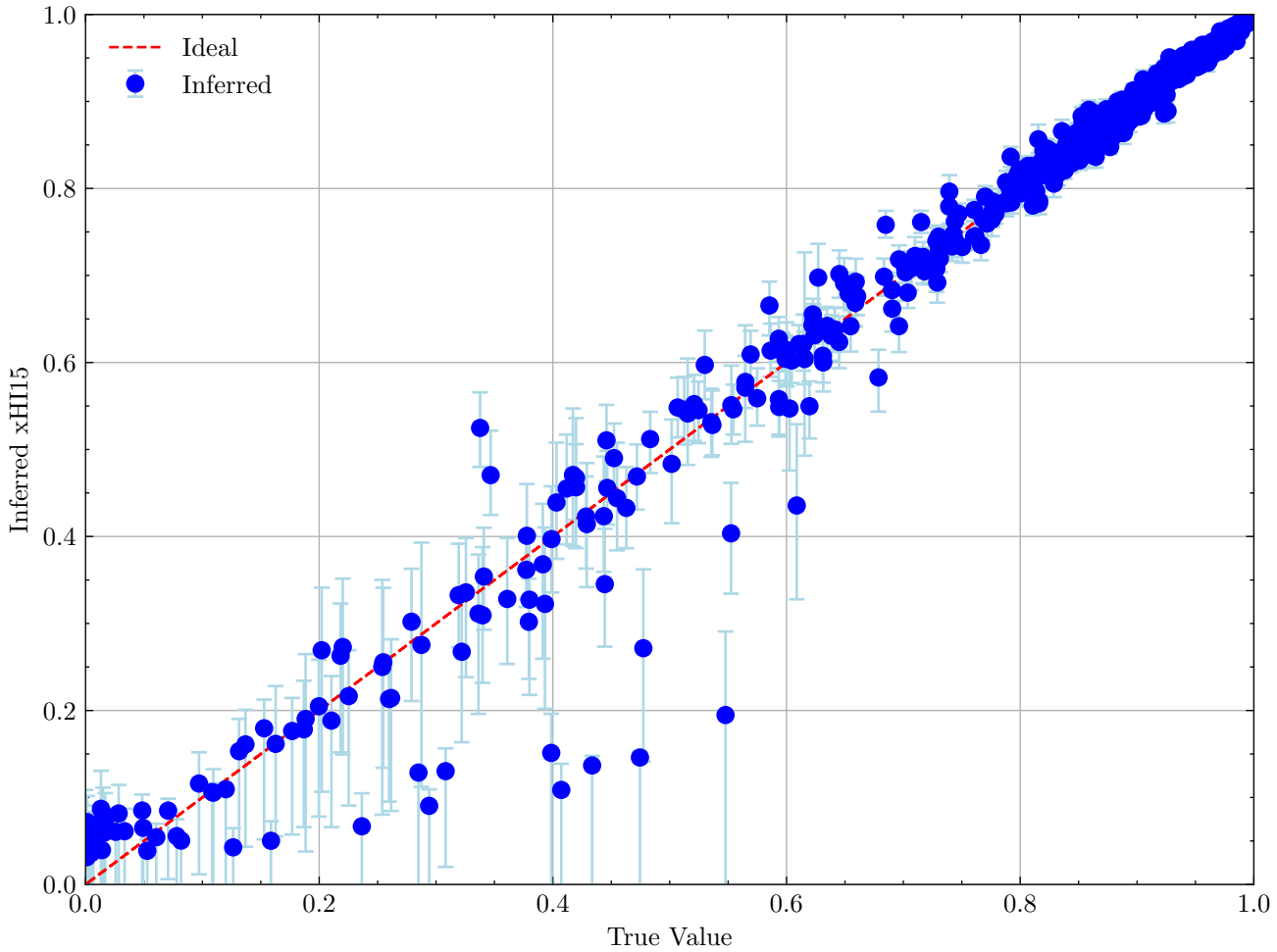
Calibration Scatter Plot for xHI15
