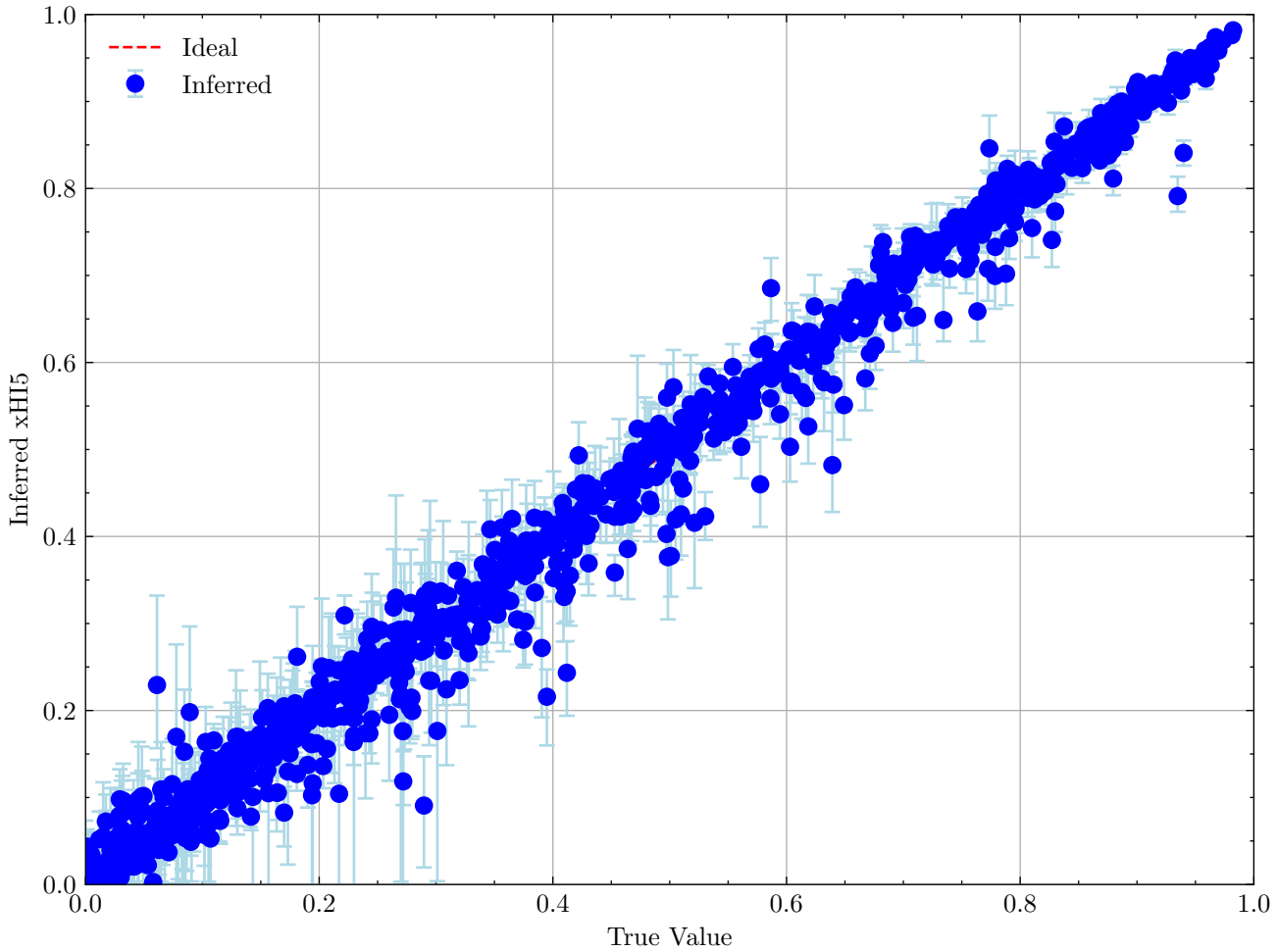
Calibration Scatter Plot for xHI5
