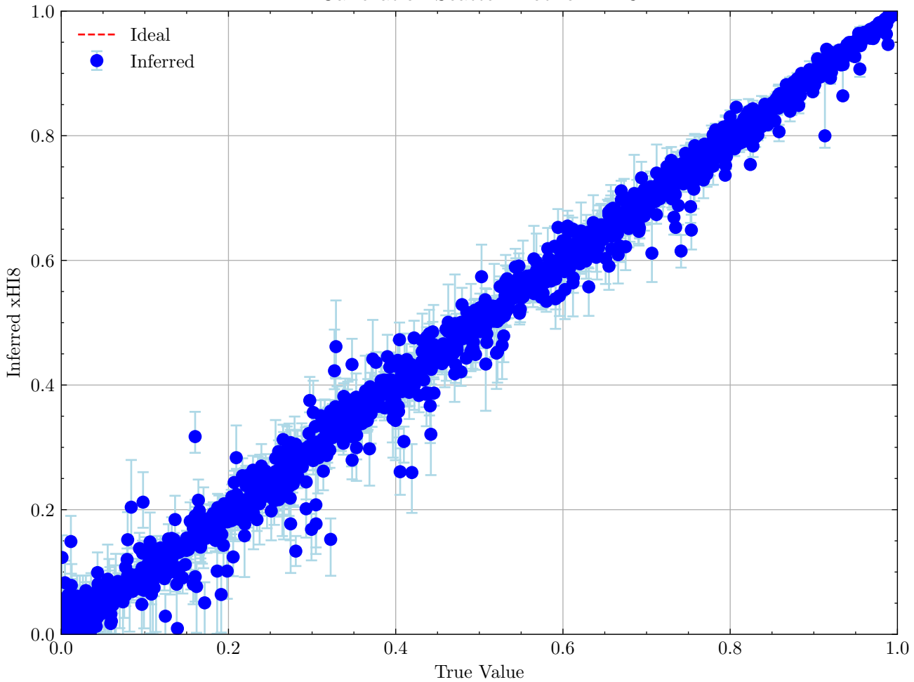
Calibration Scatter Plot for xHI8
