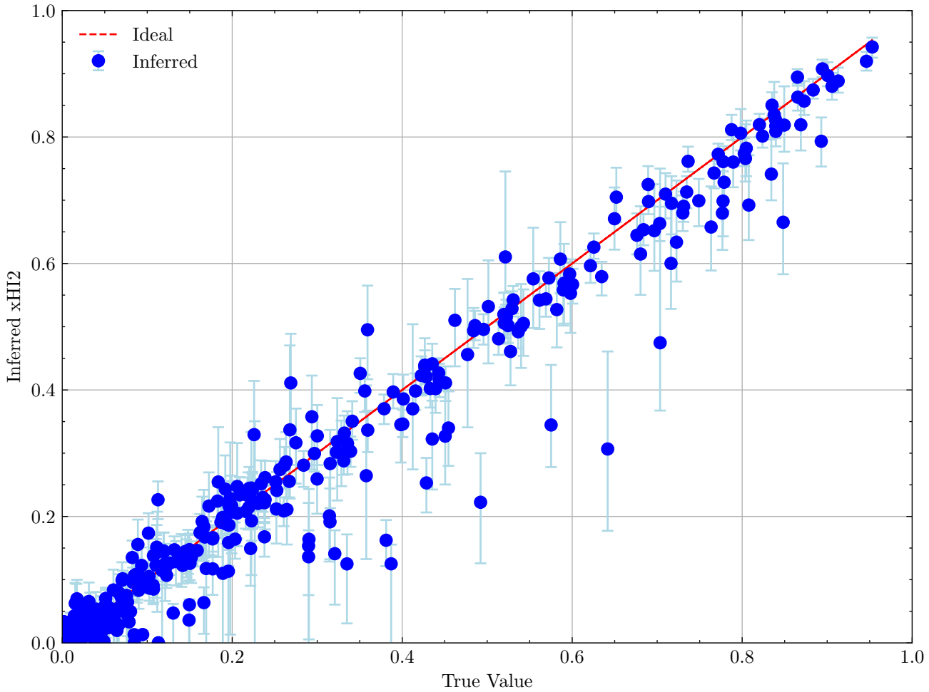
Calibration Scatter Plot for xHI2
