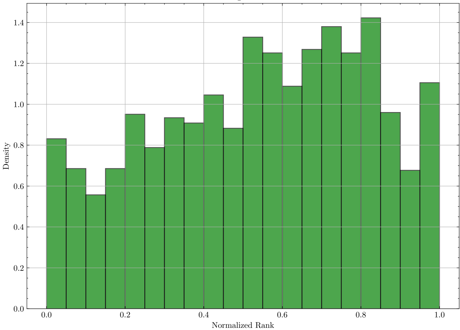
Rank Histogram for xHI7
