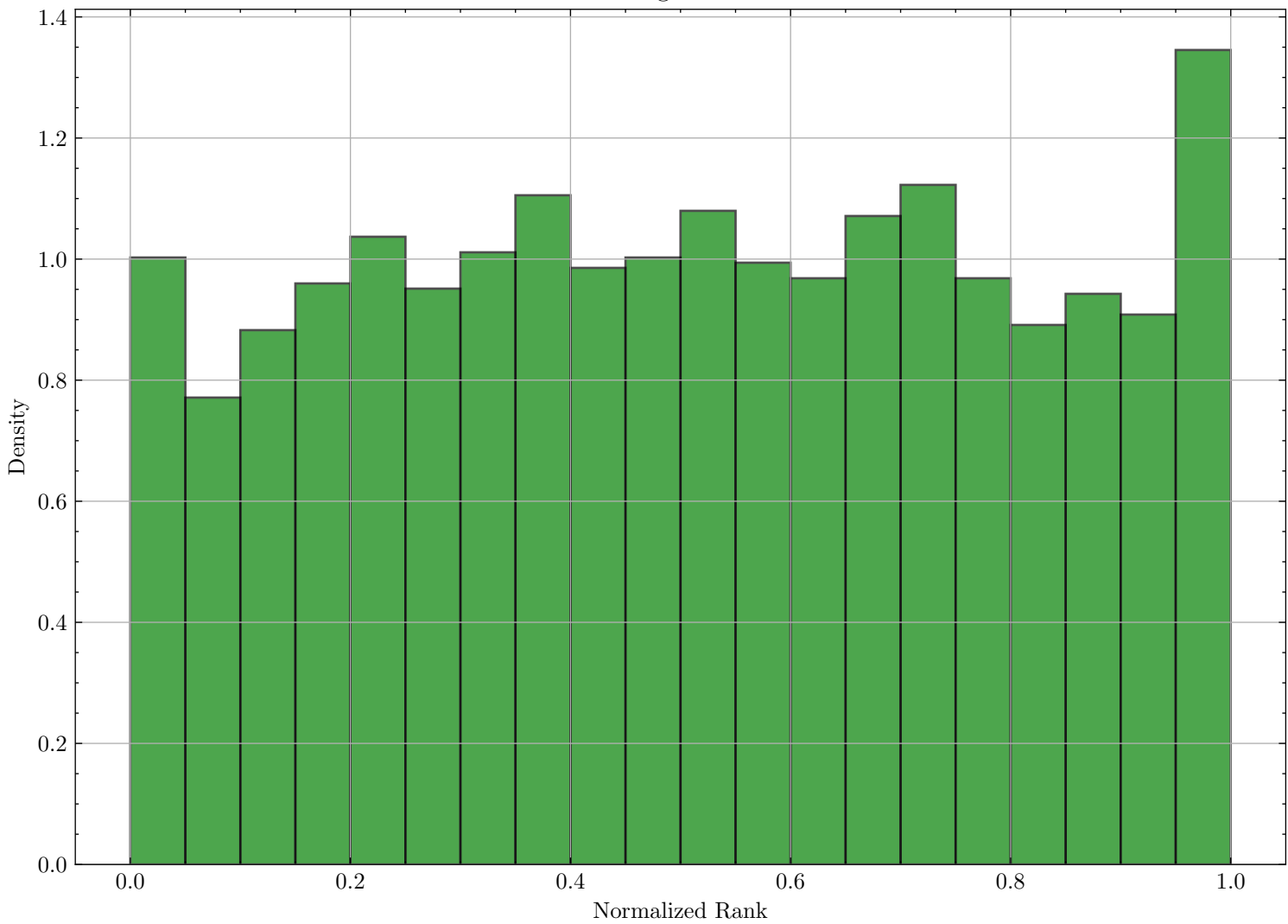
Rank Histogram for xHI14
