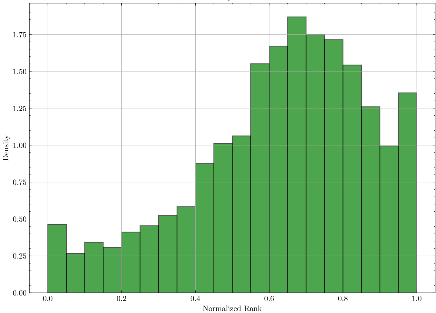
Rank Histogram for xHI3
