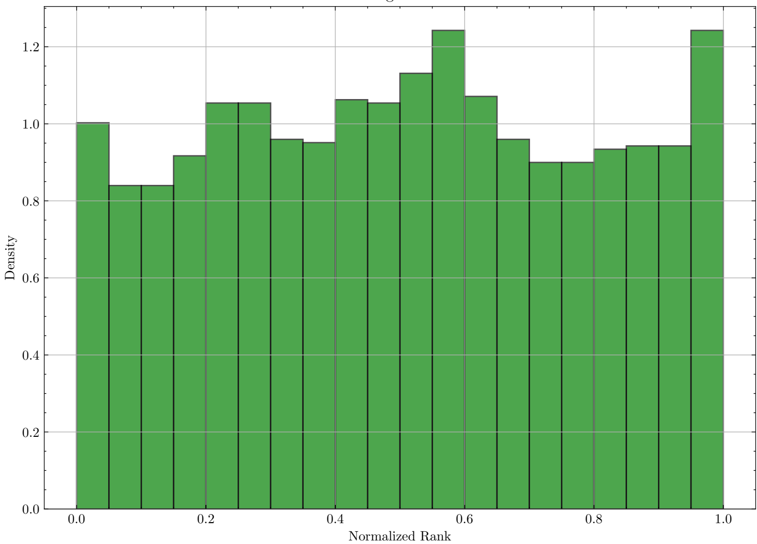
Rank Histogram for xHI13
