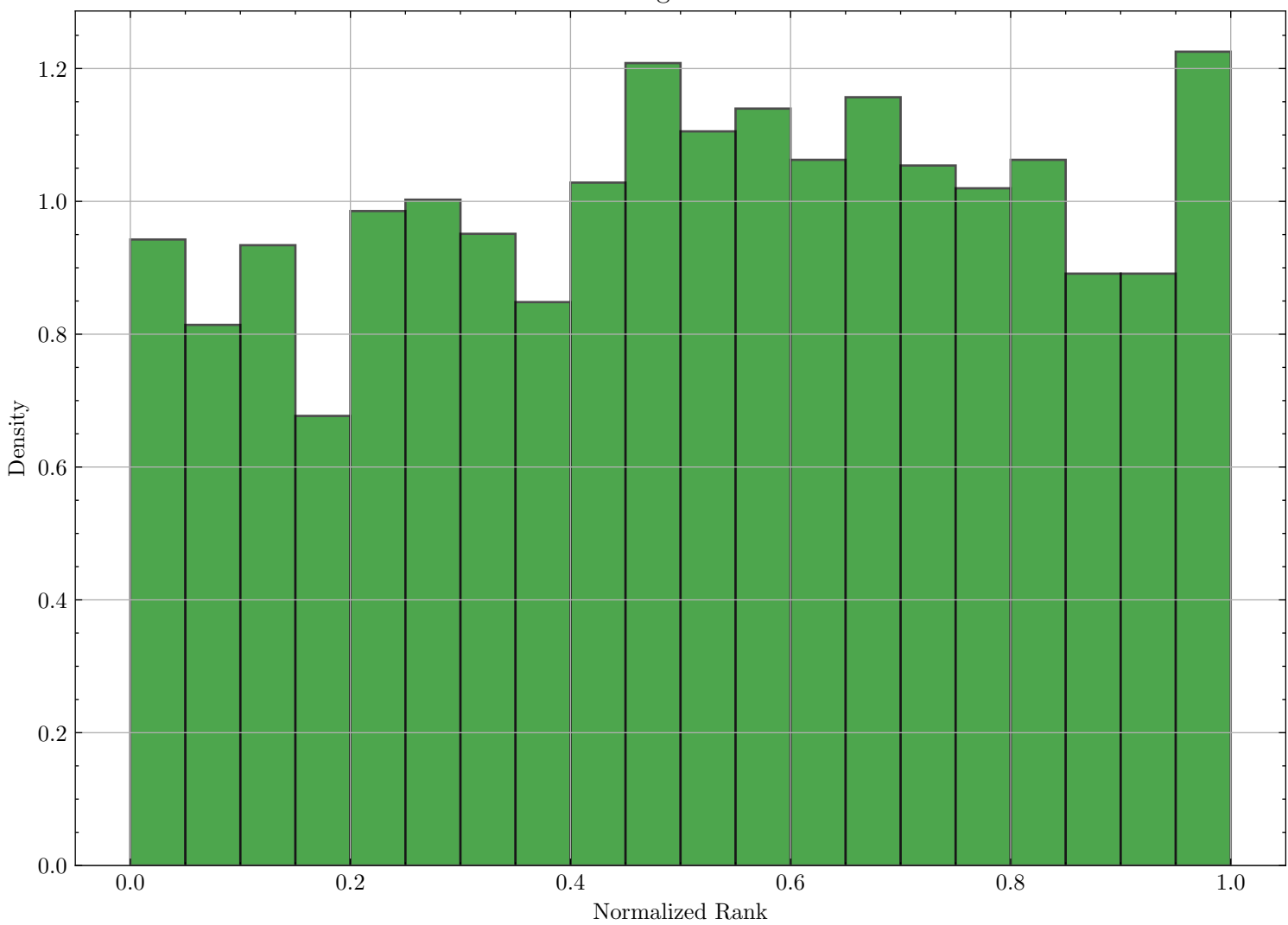
Rank Histogram for xHI10
