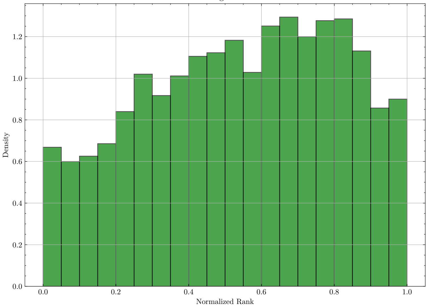
Rank Histogram for xHI6
