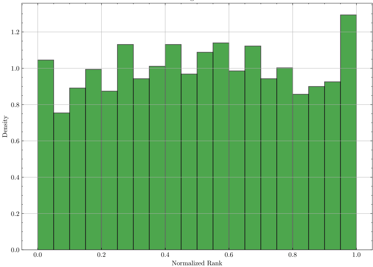
Rank Histogram for xHI15
