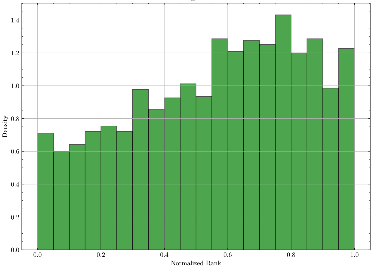
Rank Histogram for xHI8
