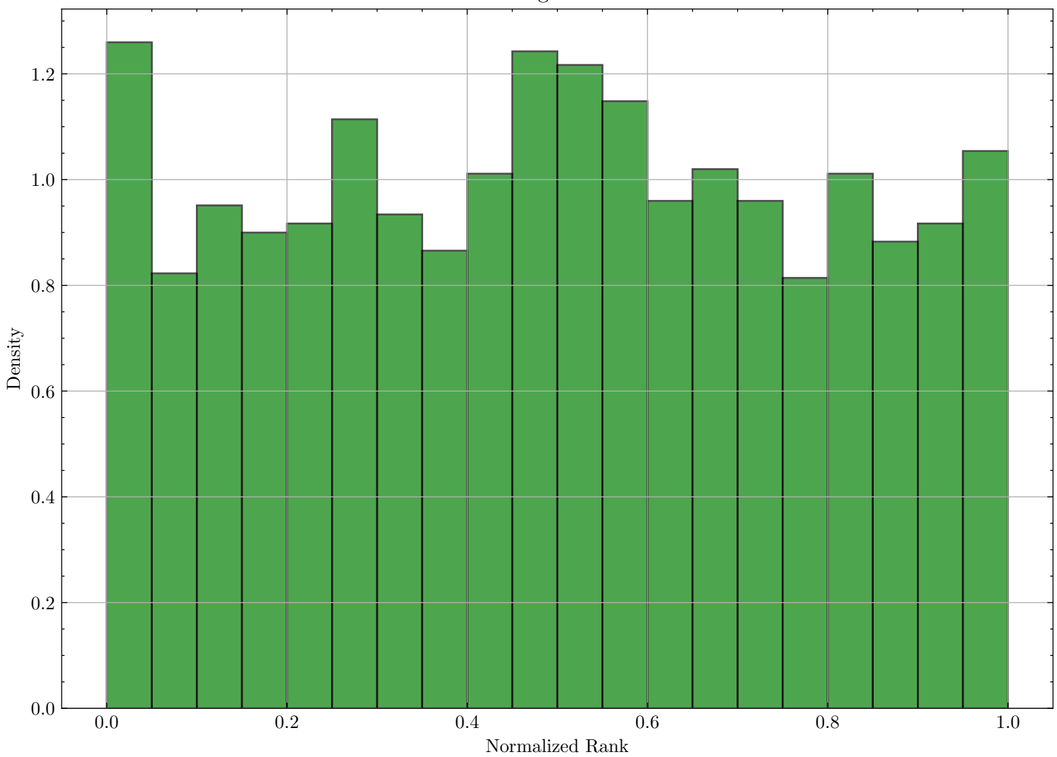
Rank Histogram for xHI11
