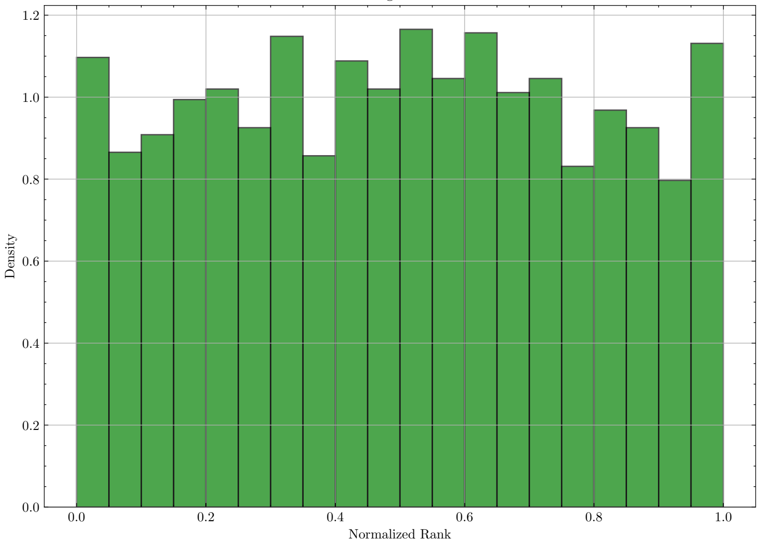
Rank Histogram for xHI12
