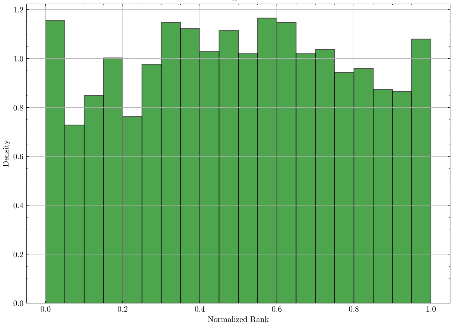
Rank Histogram for xHI9
