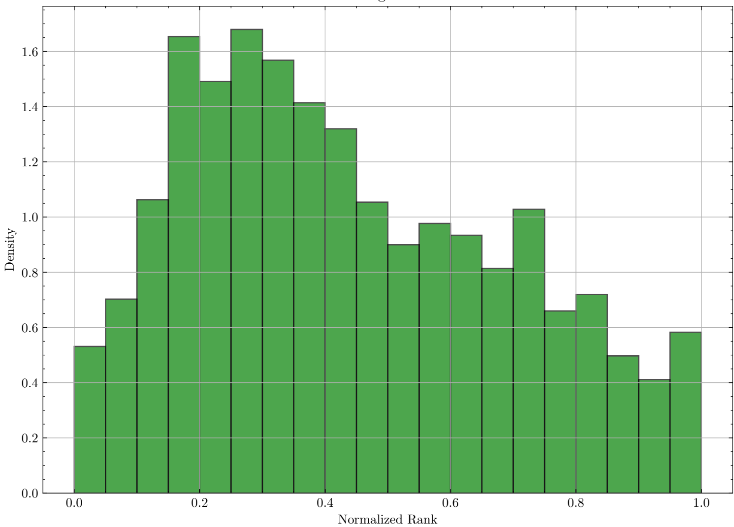
Rank Histogram for xHI1
