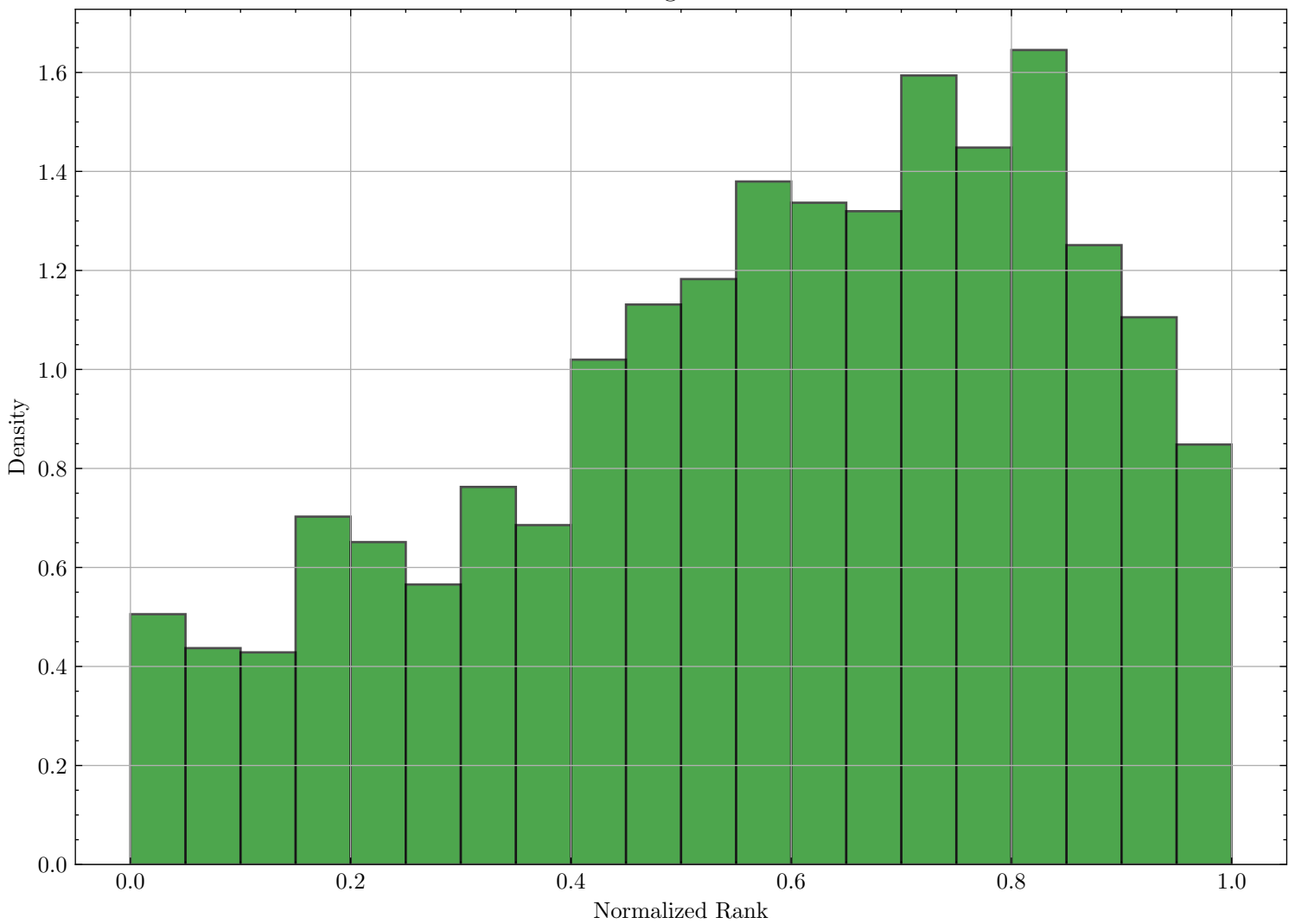
Rank Histogram for xHI4
