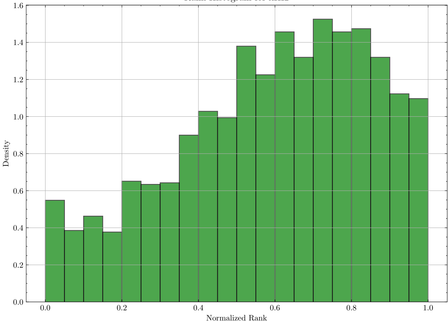
Rank Histogram for xHI2
