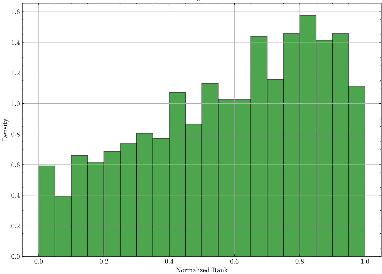
Rank Histogram for xHI5
