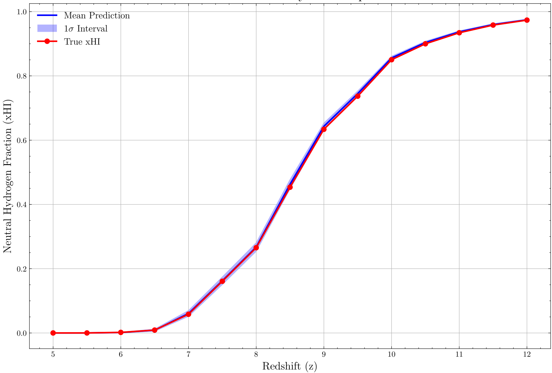
Reionization History for Example 3
