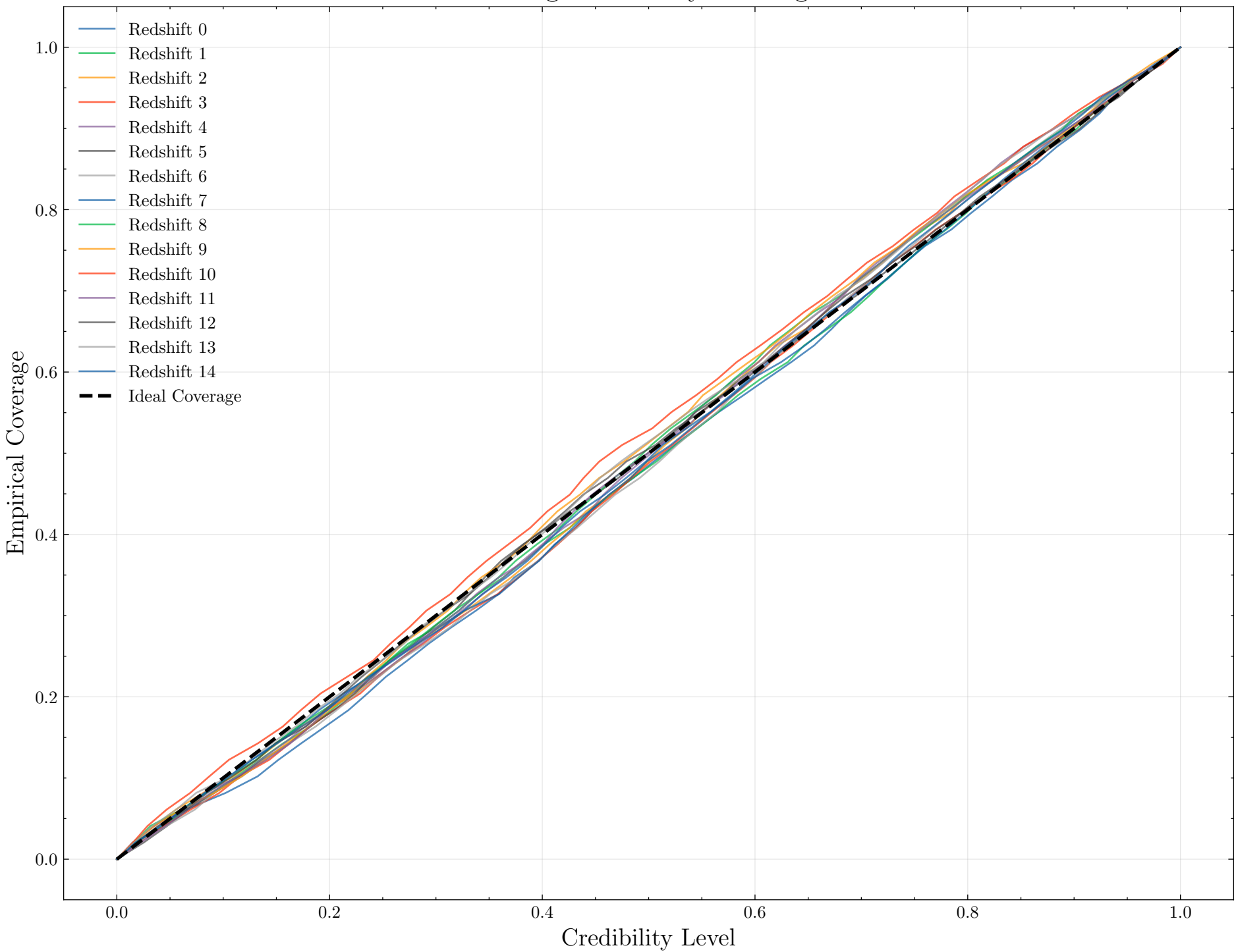
Per-Parameter Log Probability Coverage Calibration
