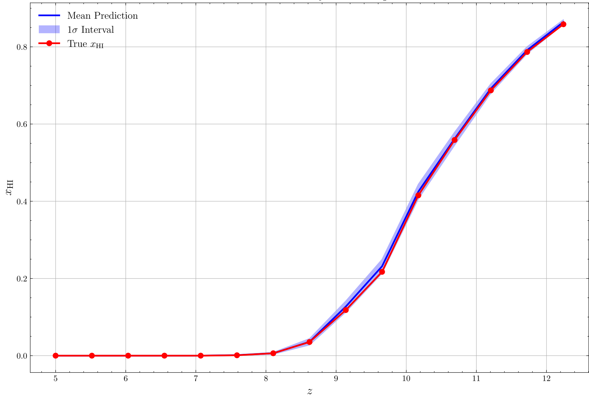
Reionization History for Example 1
