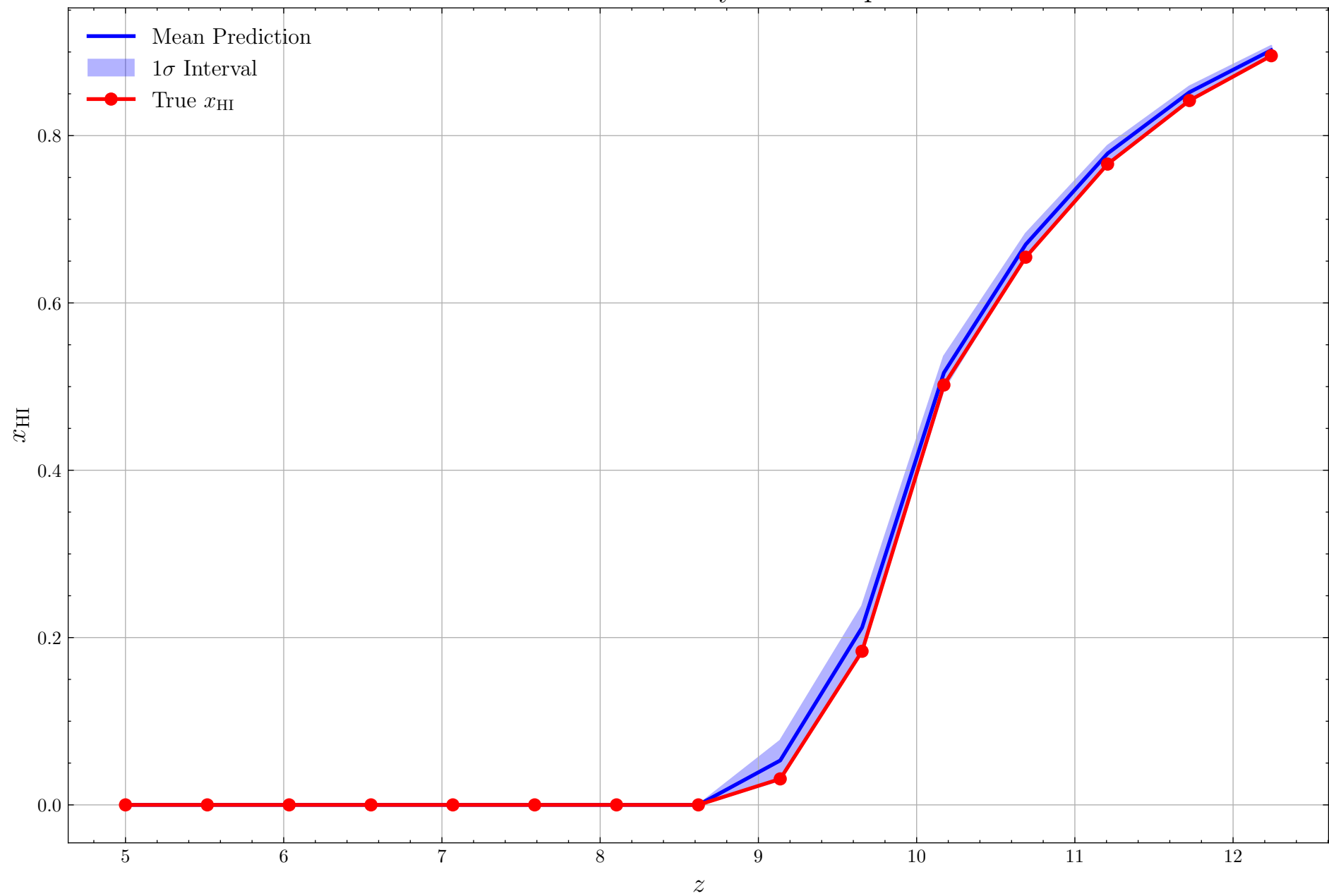
Reionization History for Example 2
