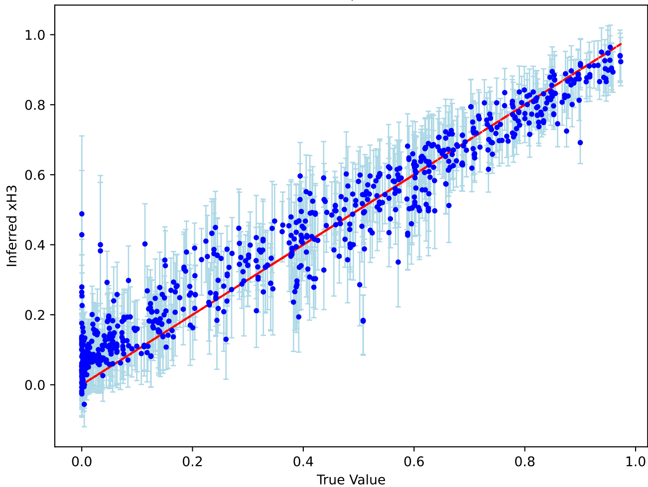
Calibration plot for xH3
