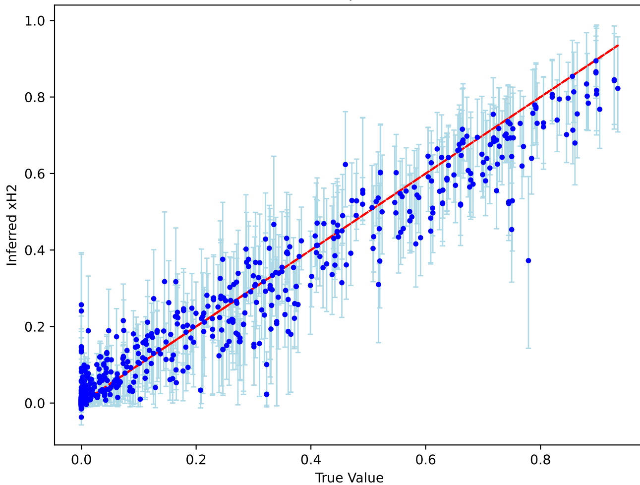
Calibration plot for xH2
