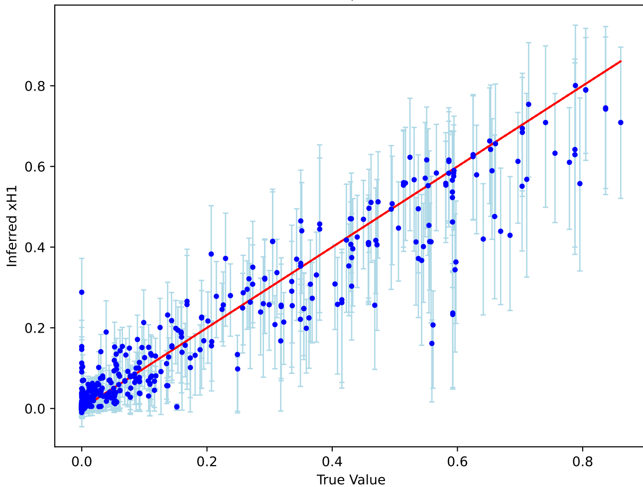
Calibration plot for xH1
