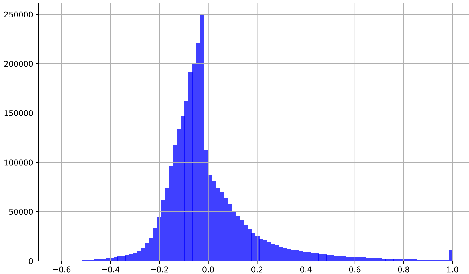
Distribution Power Spectrum
