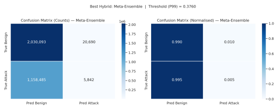
Fig. 4: Meta-Ensemble confusion matrix (P99 threshold). The ensemble detects only 5,842 of 1,164,327 attack flows (recall \approx 0.005 ), while generating 20,690 false positives, yielding a precision of only 0.2202.
