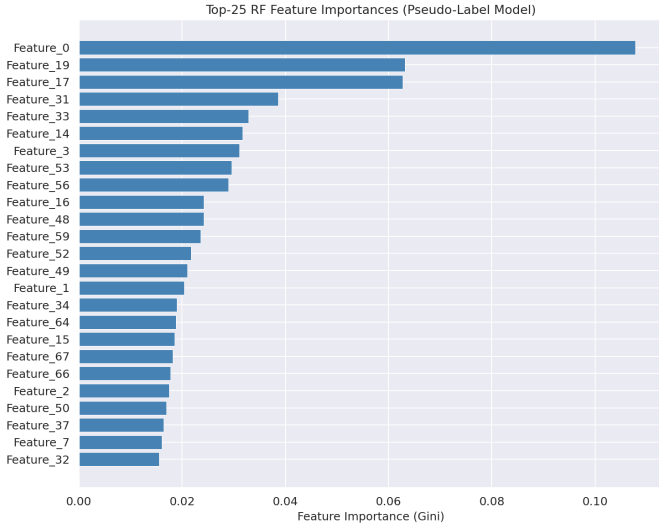
Fig. 7: RF feature importance from the pseudo-label classifier. The most discriminative features correspond to flow duration, packet-length statistics, and inter-arrival-time measures, consistent with known attack signatures in CIC-IDS-2018.
