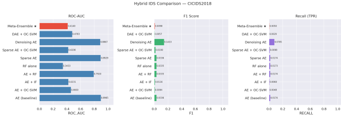
Fig. 3: F1 / ROC-AUC / Recall comparison across all models. Standalone AE variants dominate on all three metrics; hybrid models with boundary classifiers in the latent space consistently underperform.
