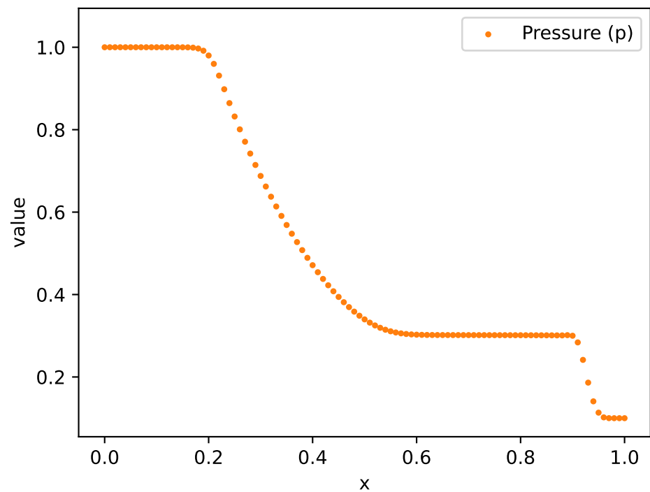
Test Cartesian shock tube problem at t=0.245 with 100 grid points
