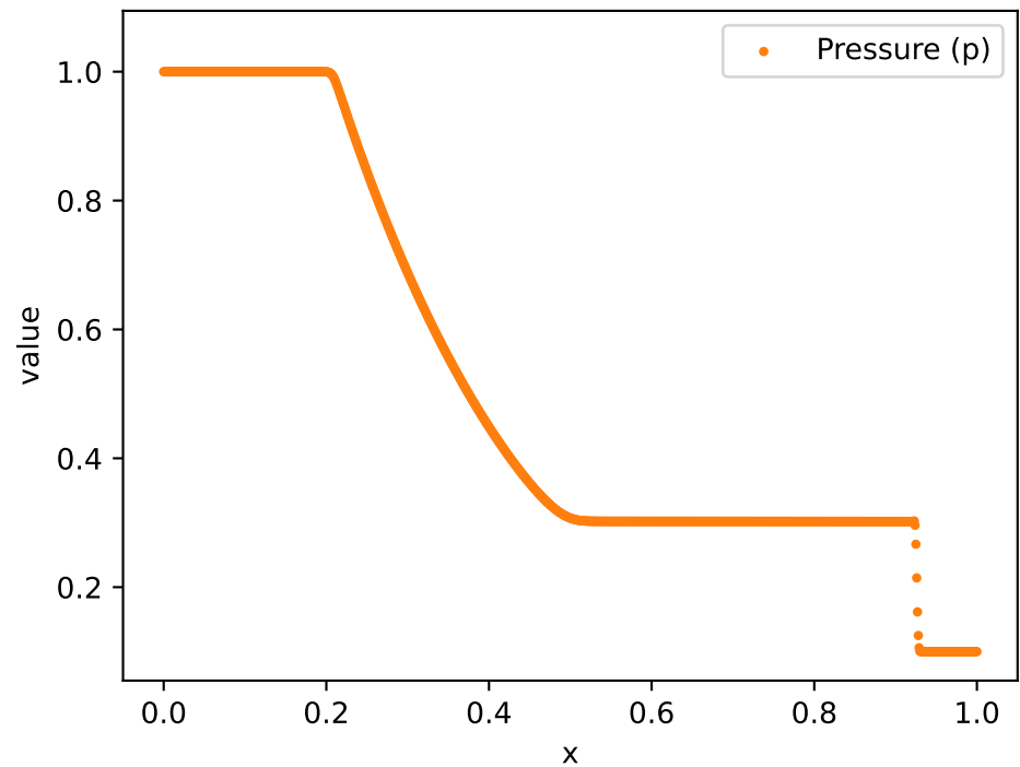
Test Cartesian shock tube problem at t=0.245 with 1000 grid points
