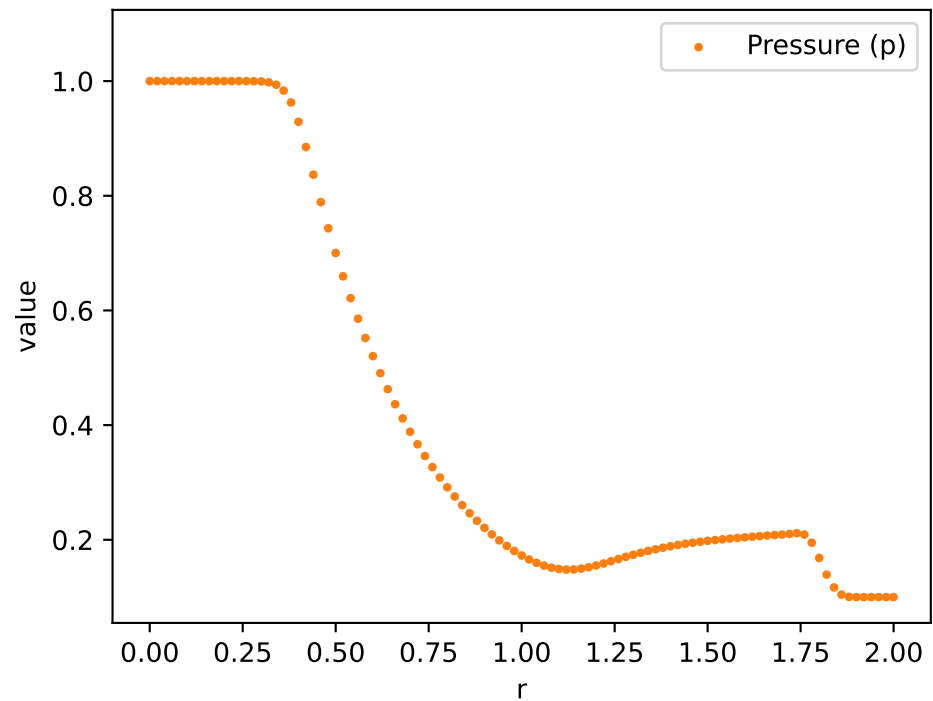
Test spherical shock tube problem at t=0.5 with 100 grid points
