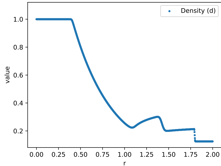
Test spherical shock tube problem at t=0.5 with 1000 grid points
