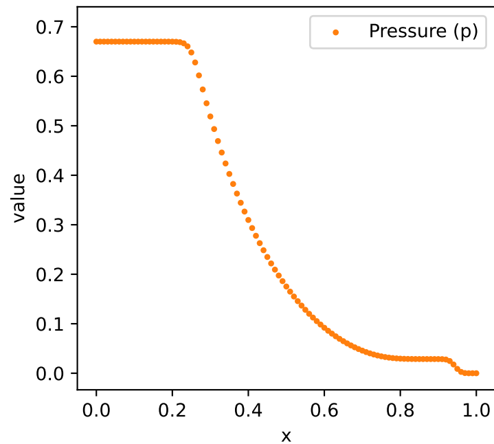
Strong shock tube at t=2.3 with 100 grid points
