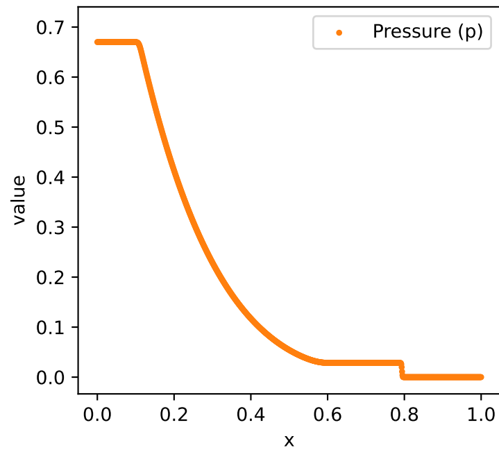
Strong shock tube at t=2.3 with 1000 grid points
