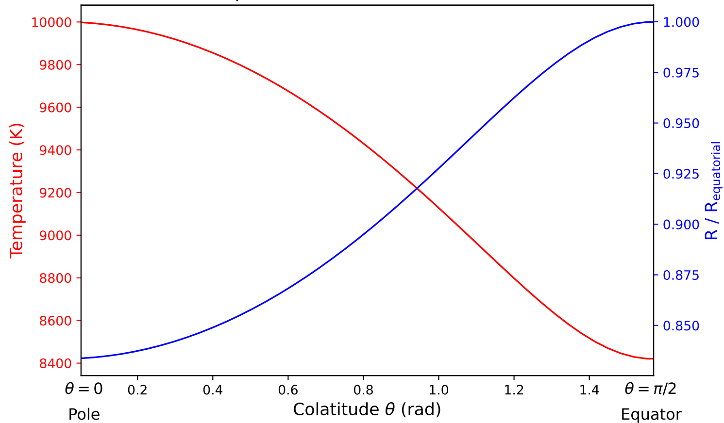
Temperature and radius vs colatitude
