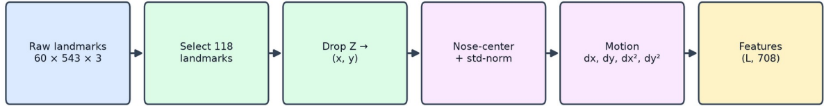
Figure 4.2: ASL preprocessing
