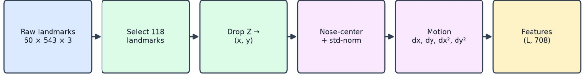
Figure 4.2: ASL preprocessing
