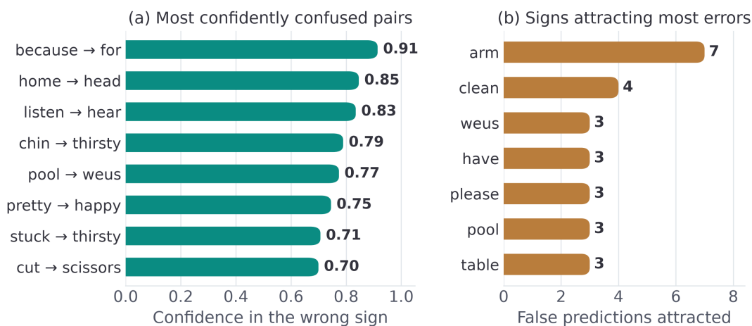
Figure 5.3: ASL confusion analysis (most-confused sign pairs)
