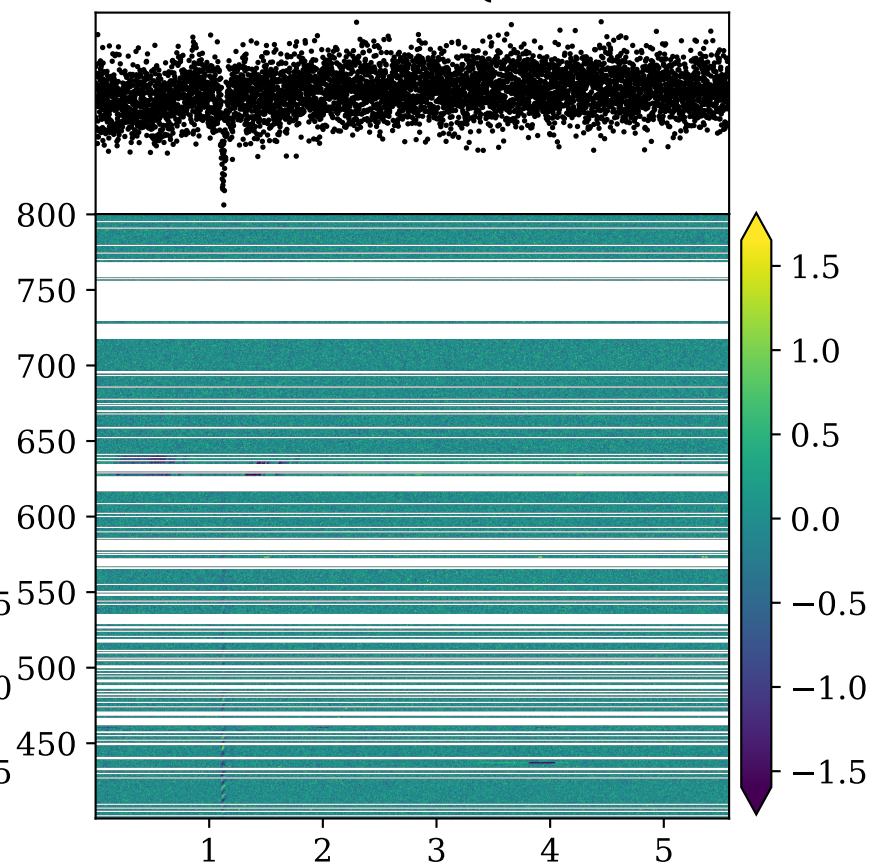
Stokes V
