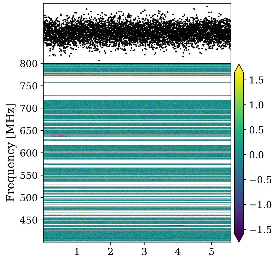
Stokes U
