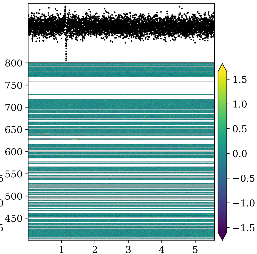
Stokes V
