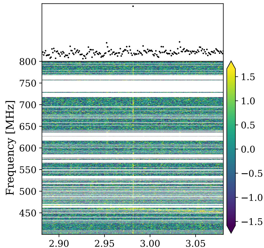
Stokes U
