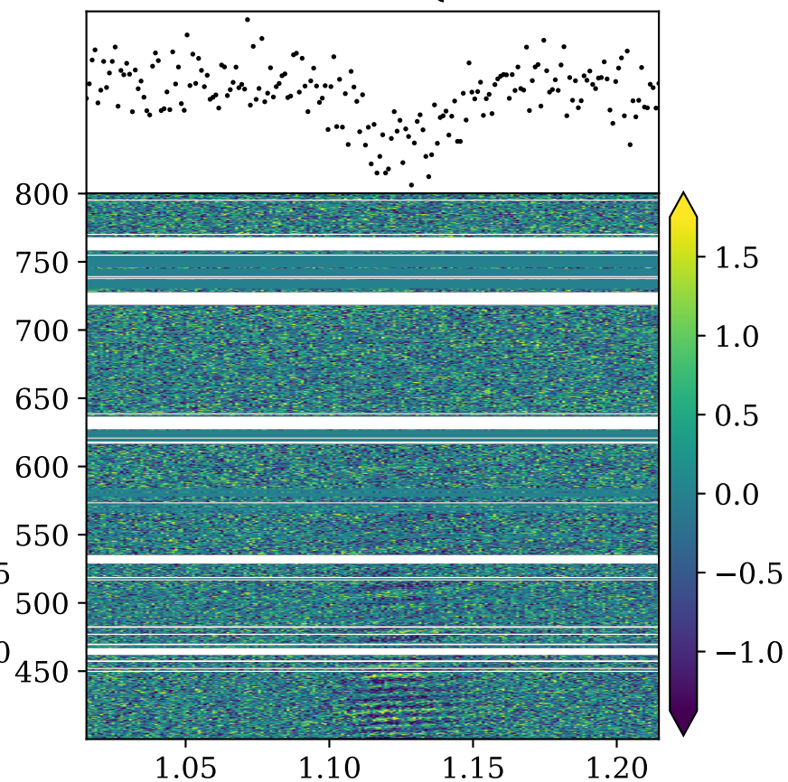
Stokes V
