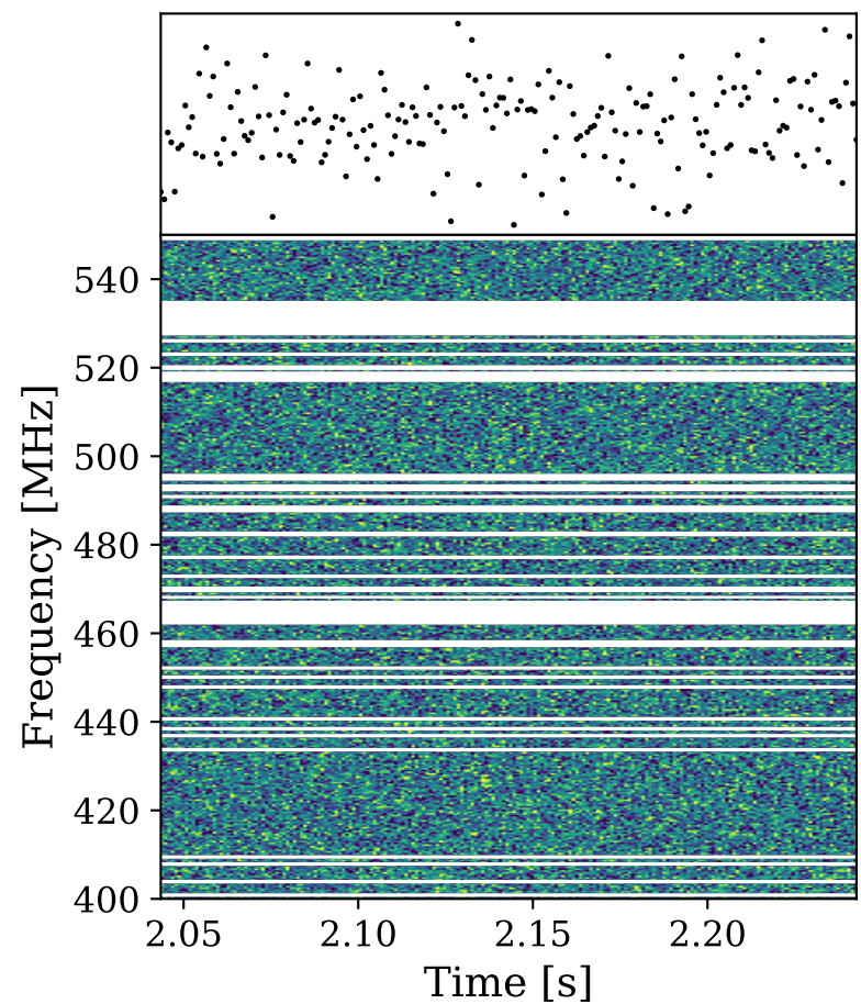
Stokes U
