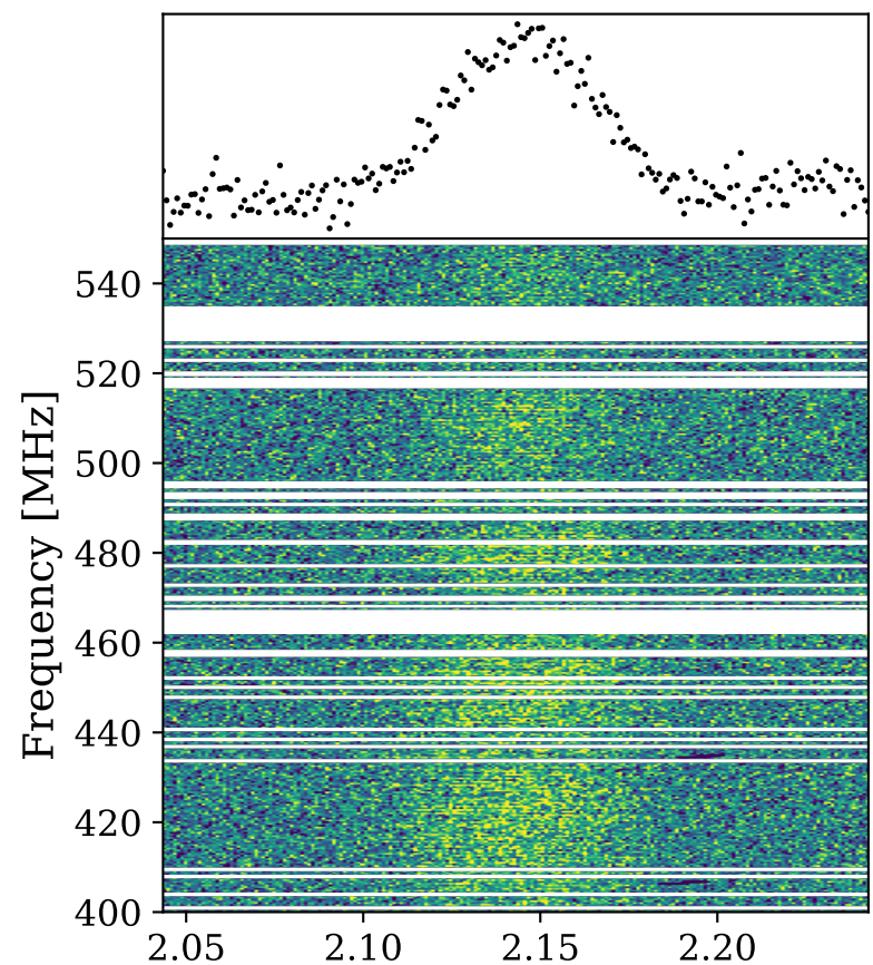
Stokes U
