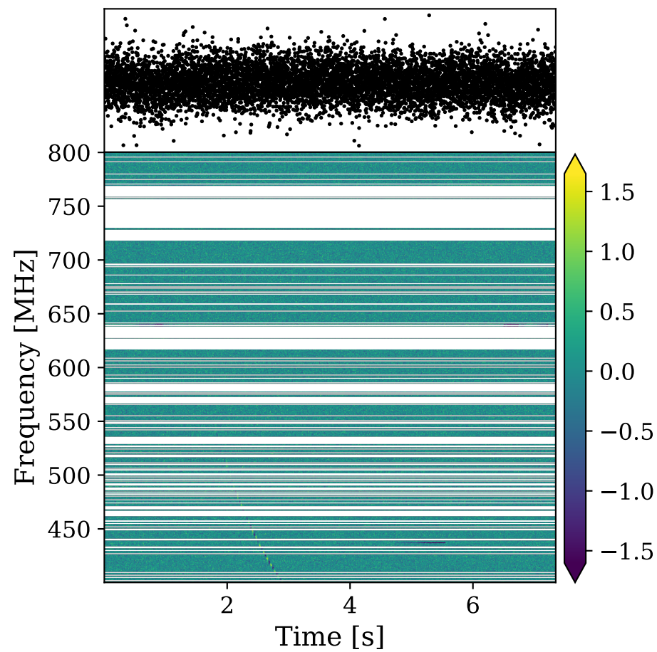
Stokes U
