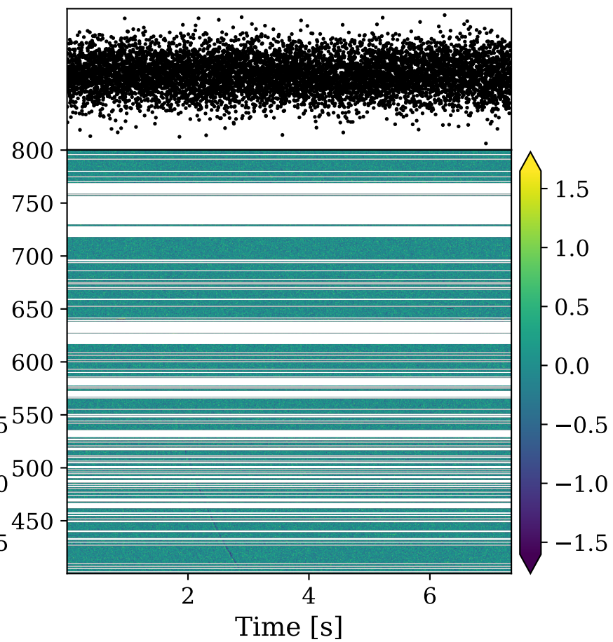
Stokes V
