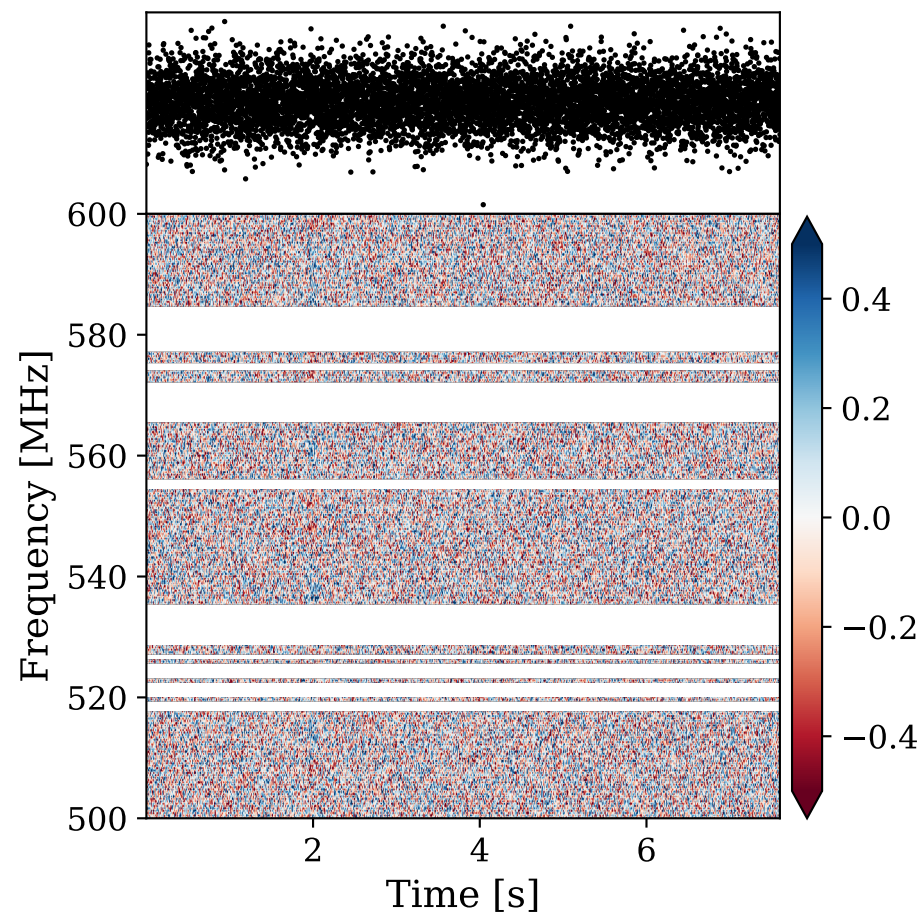
Stokes U
