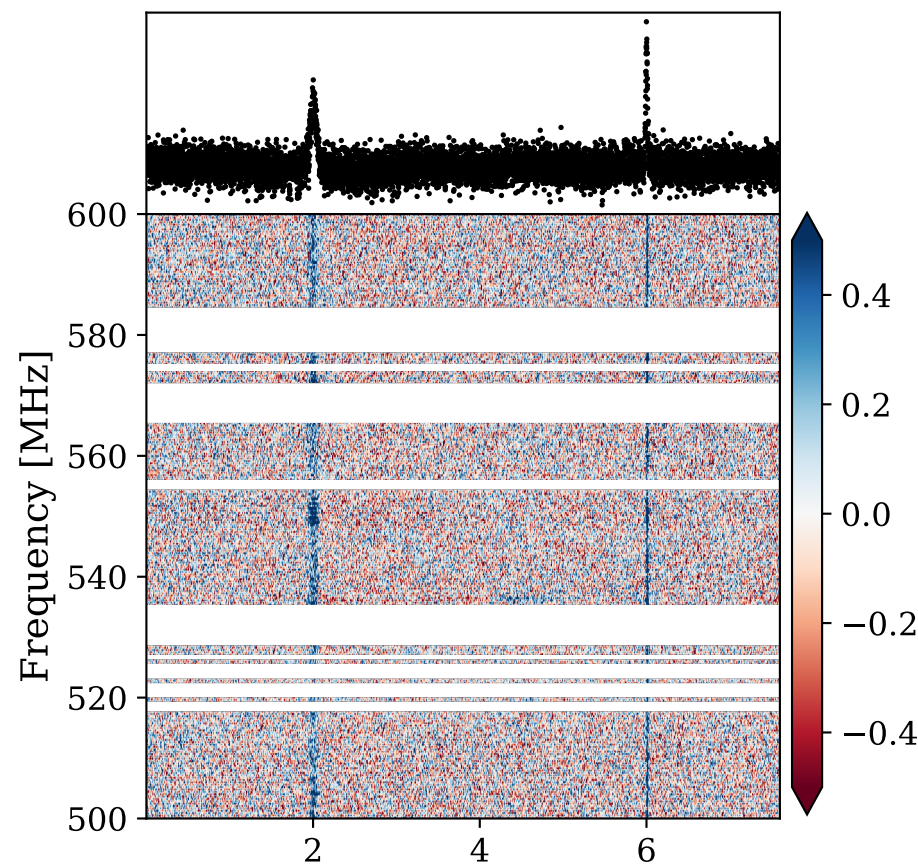
Stokes U
