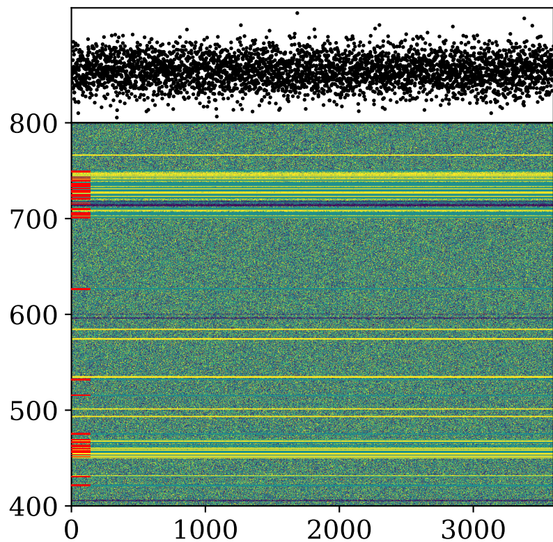
Stokes V
