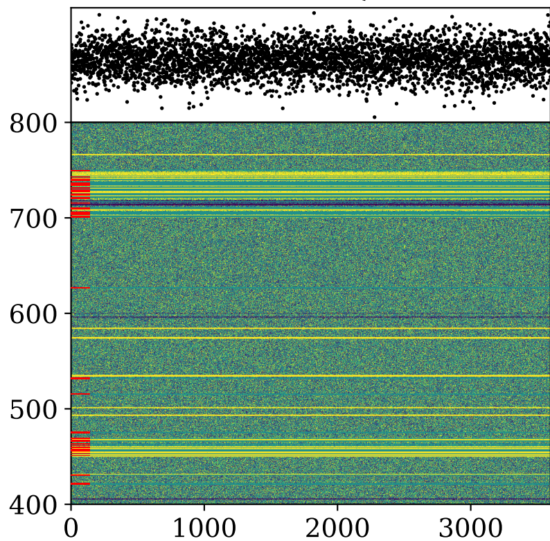
Stokes Q
