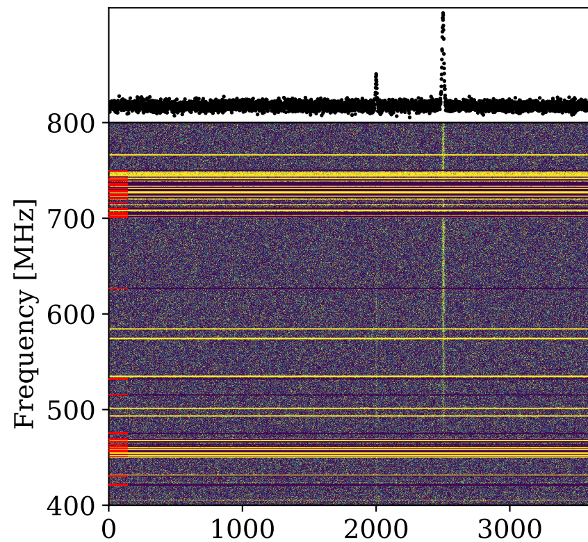
Stokes I
