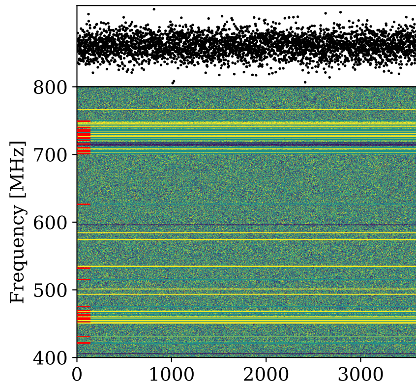
Stokes U
