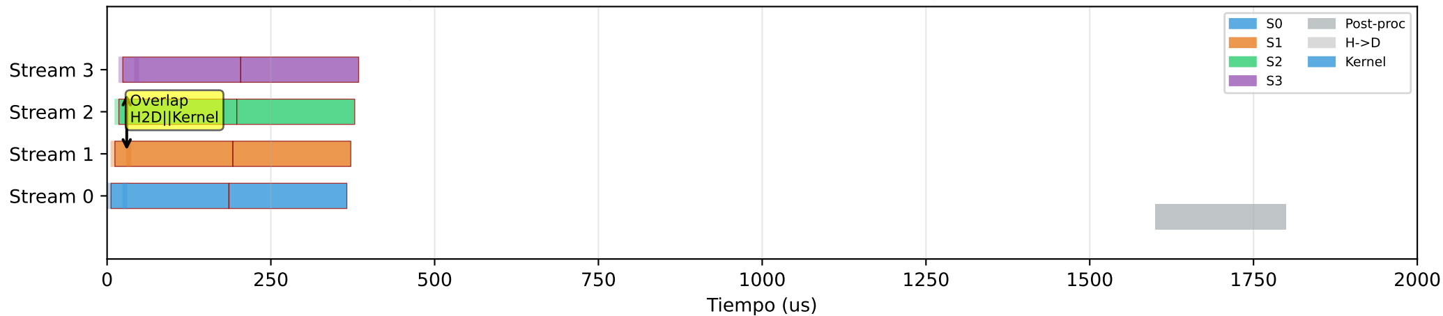
Experimento 2: S=4 streams con double buffering, Total = 1.829 ms
