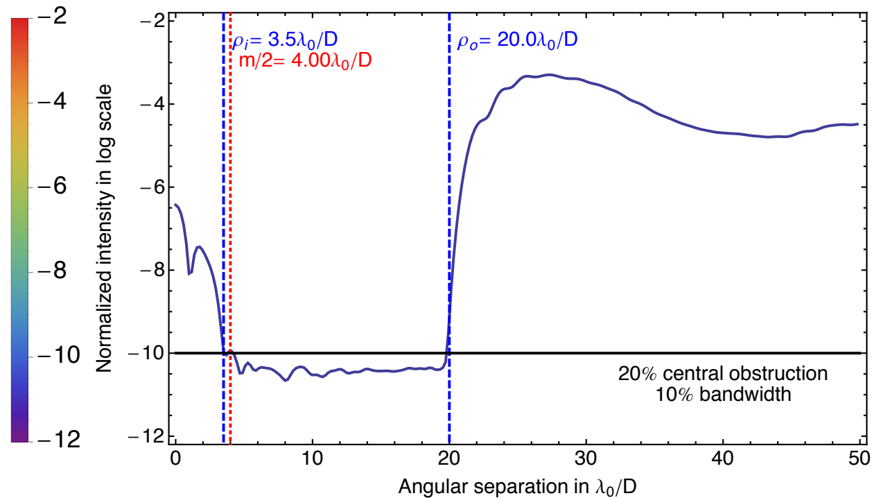
Radial profile of the coronagraphic image for a spectral band \lambda/\Delta\lambda=10\%
