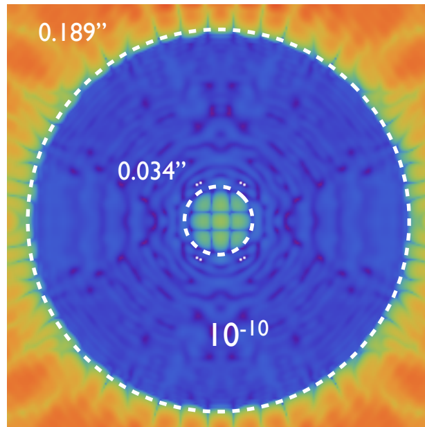
Coronagraphic image for a spectral band \lambda/\Delta\lambda=10\%
