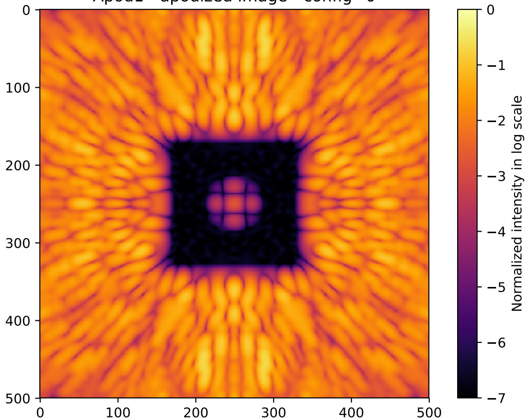
Apod1 - apodized image - config=0
