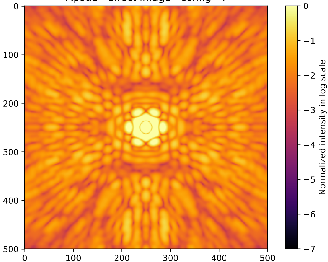
Apod1 - direct image - config=4
