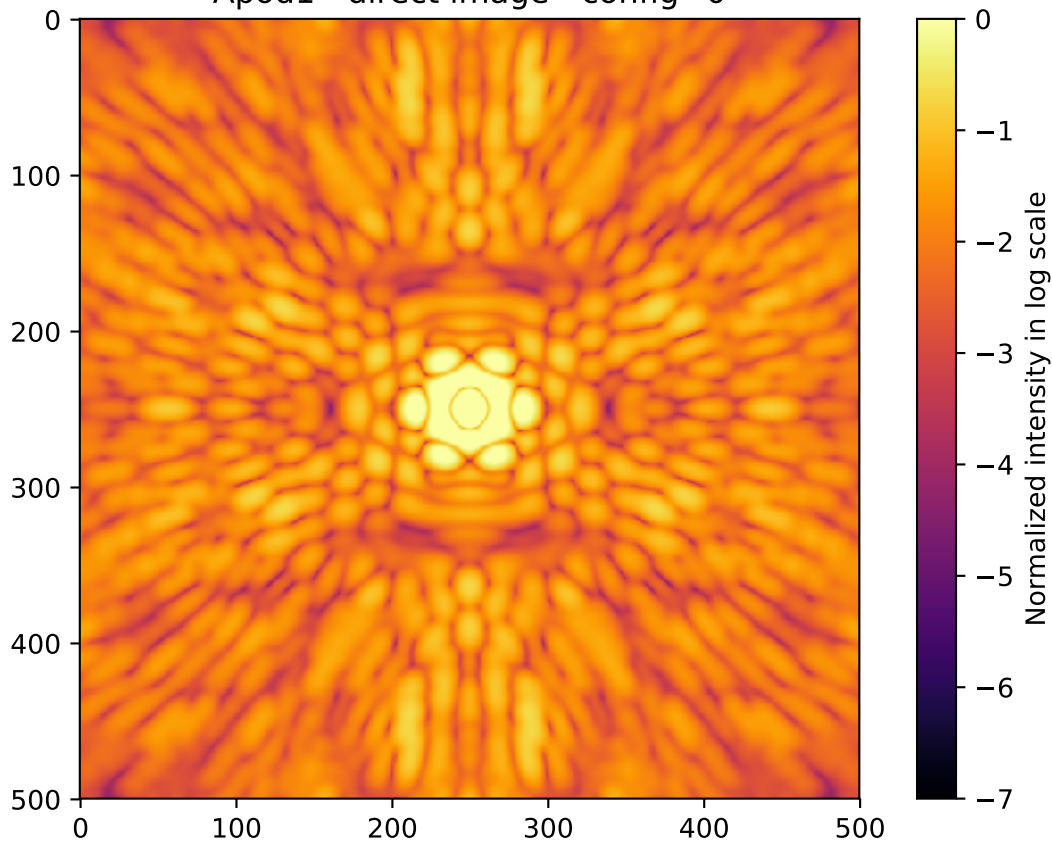
Apod1 - direct image - config=0
