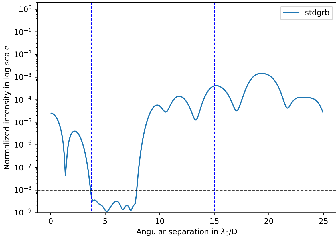
Radial intensity profiles of the images - config=0
