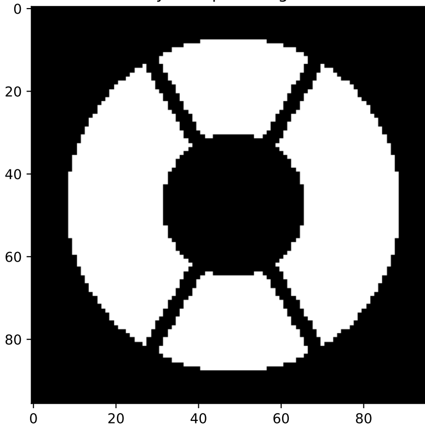
Lyot stop - config=4
