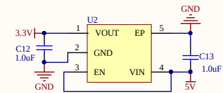
5V -> 3.3V 电源转换 5V -> 3.3V Power conversion
