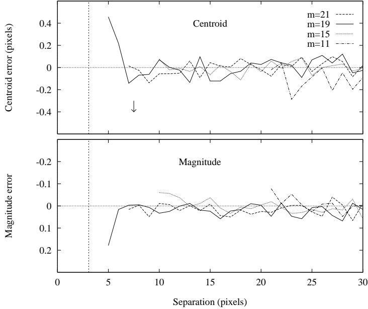
Figure 5: Centroid and corrected isophotal magnitude errors for a simulated 19^{\text{th}} magnitude star blended with a 11, 15, 19 and 21^{\text{th}} mag. companion as a function of distance (expressed in pixels). Lines stop at the left when the objects are too close to be deblended. The dashed vertical line is the theoretical limit for unsaturated stars with equal magnitudes. In the centroid plot, the arrow indicates the direction of the neighbour. The simulation assumes a 1 hour exposure with the CERGA telescope on a IIIaJ plate and Moffat profiles with a seeing FWHM of 3 pixels ( 2'' ).
