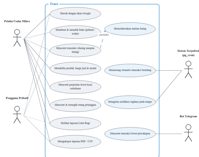
Gambar 3. Use case diagram Tracr
