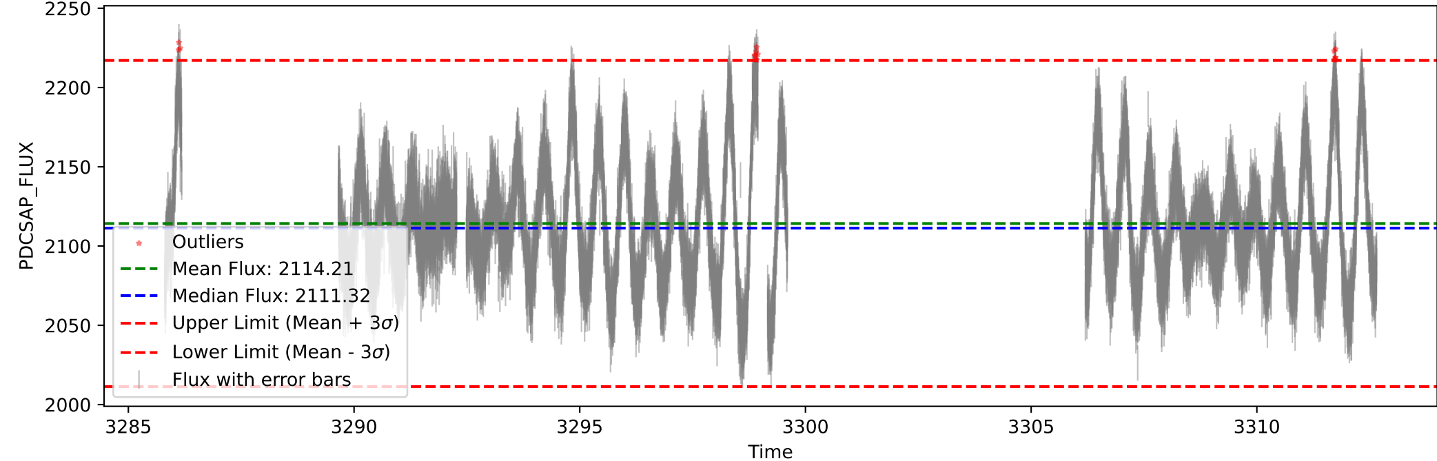
Light Curve: tess_curve_01
