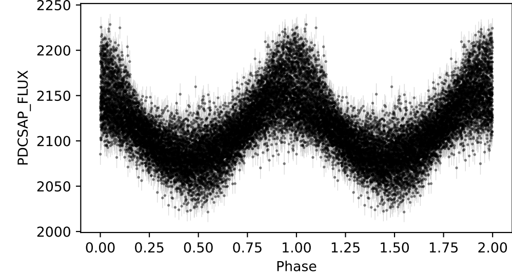
Phase-Folded Light Curve (Period = 0.5831)
