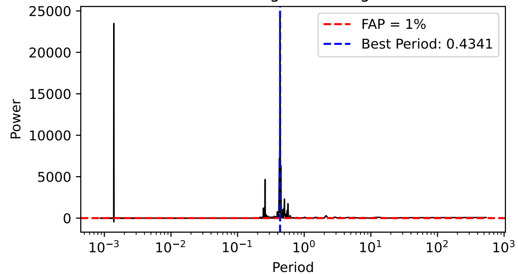
Lomb-Scargle Periodogram
