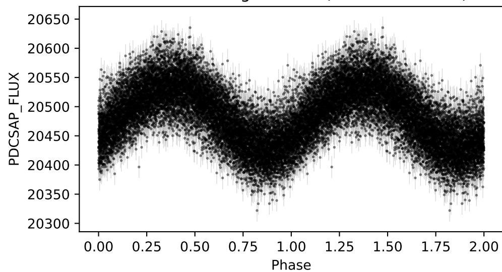
Phase-Folded Light Curve (Period = 0.4341)
