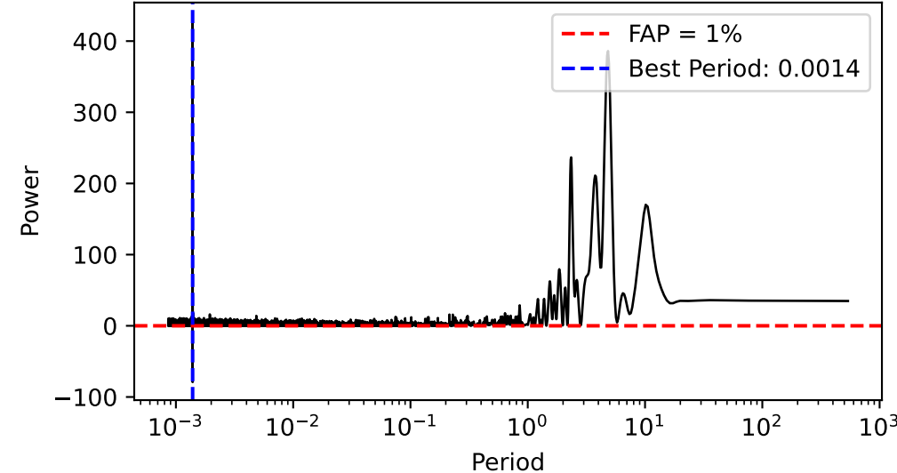
Lomb-Scargle Periodogram
